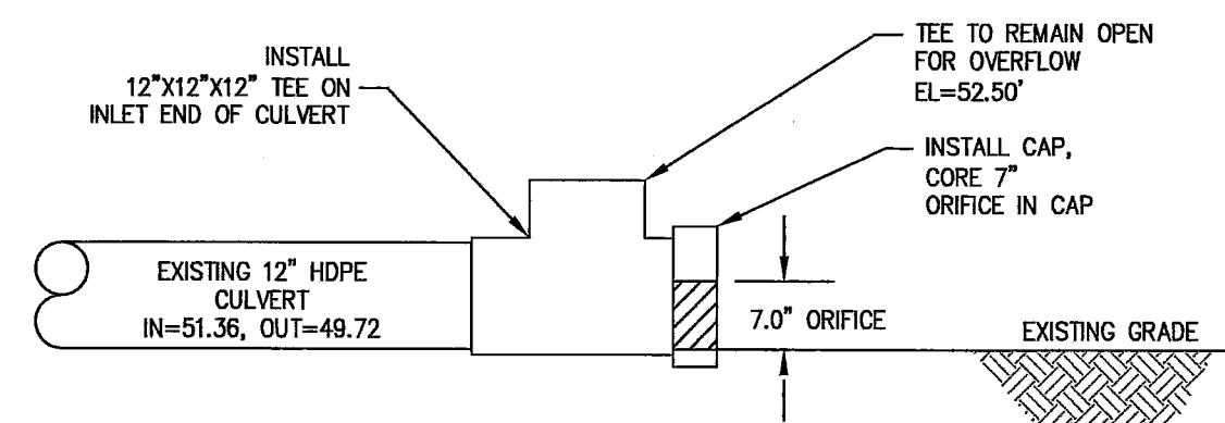
OUTLET CONTROL STRUCTURE NOT TO SCALE
