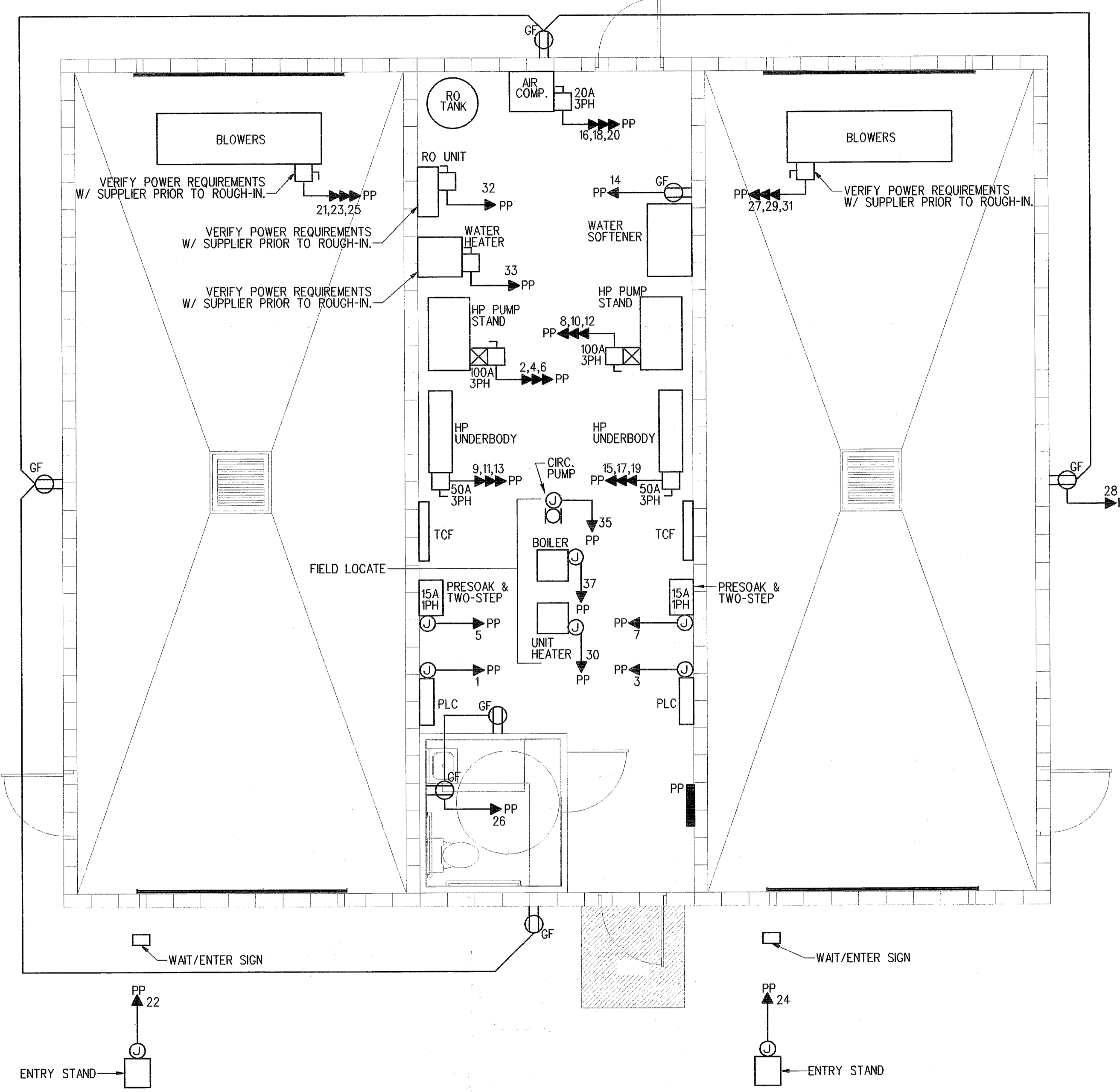
POWER PLAN SCALE: 1/4"=1'-0"
