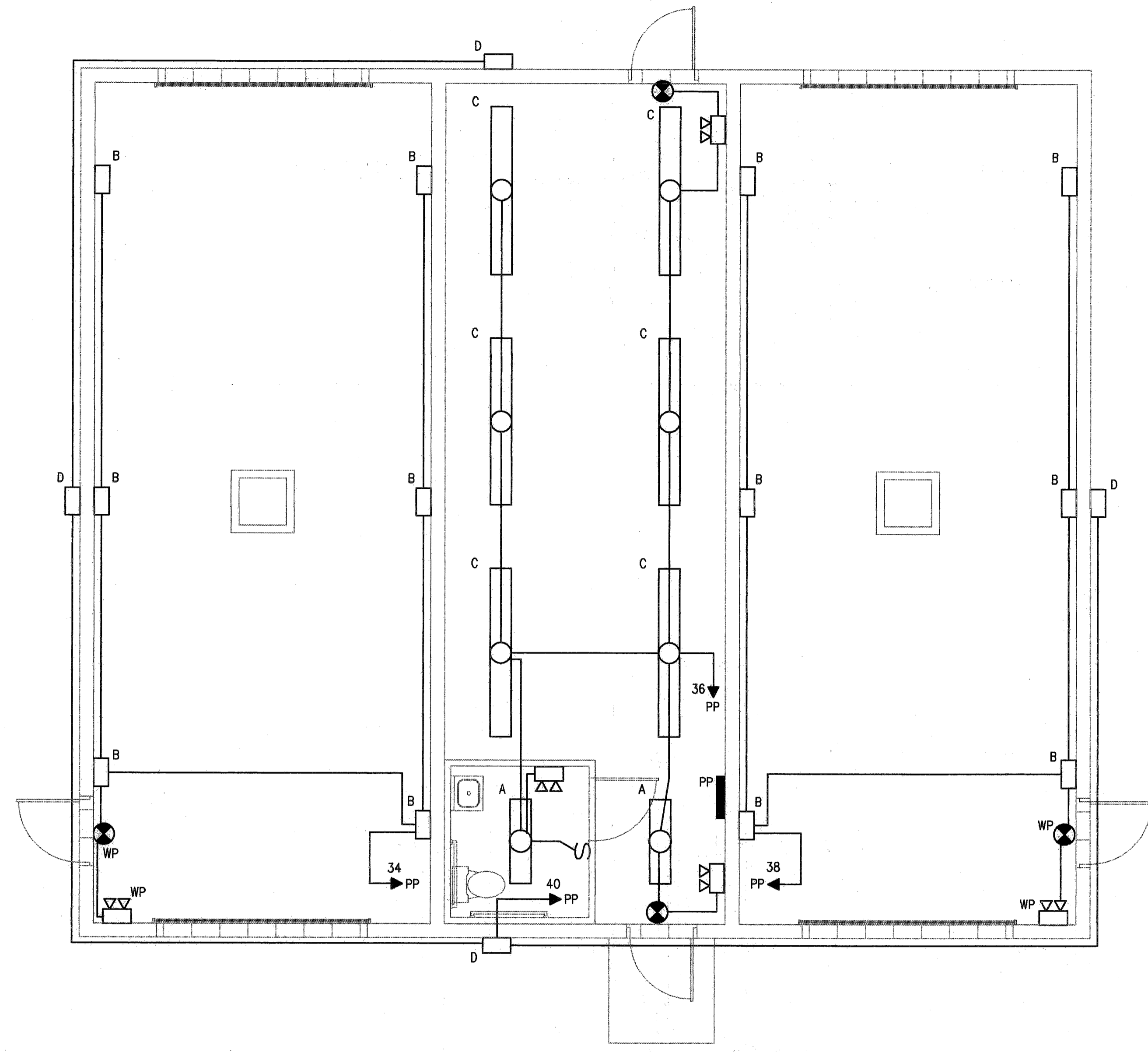
LIGHTING PLAN SCALE: 1/4"=1'-0"
