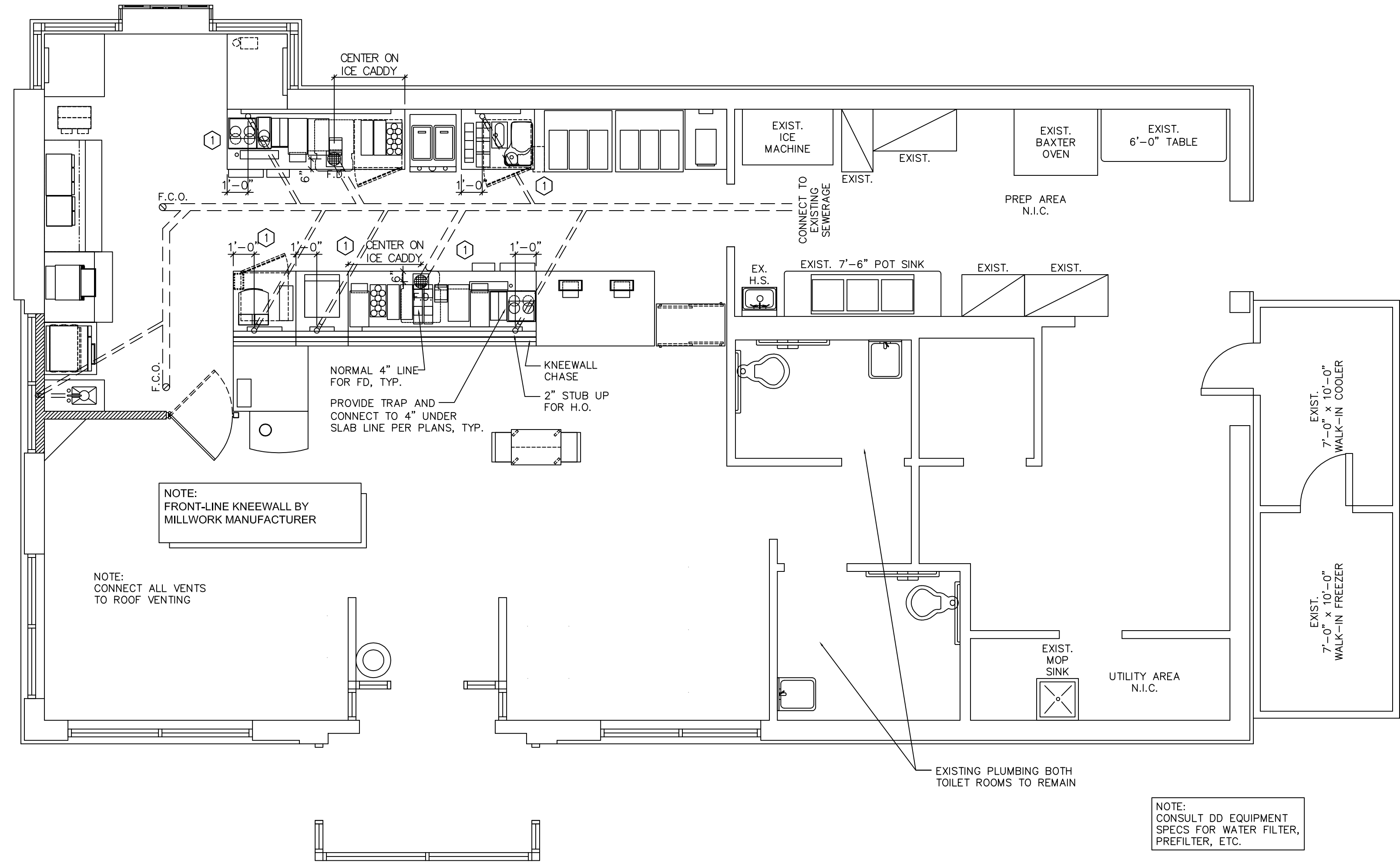
1 SOIL, WASTE & VENT PLAN 1/4"=1'-0"
