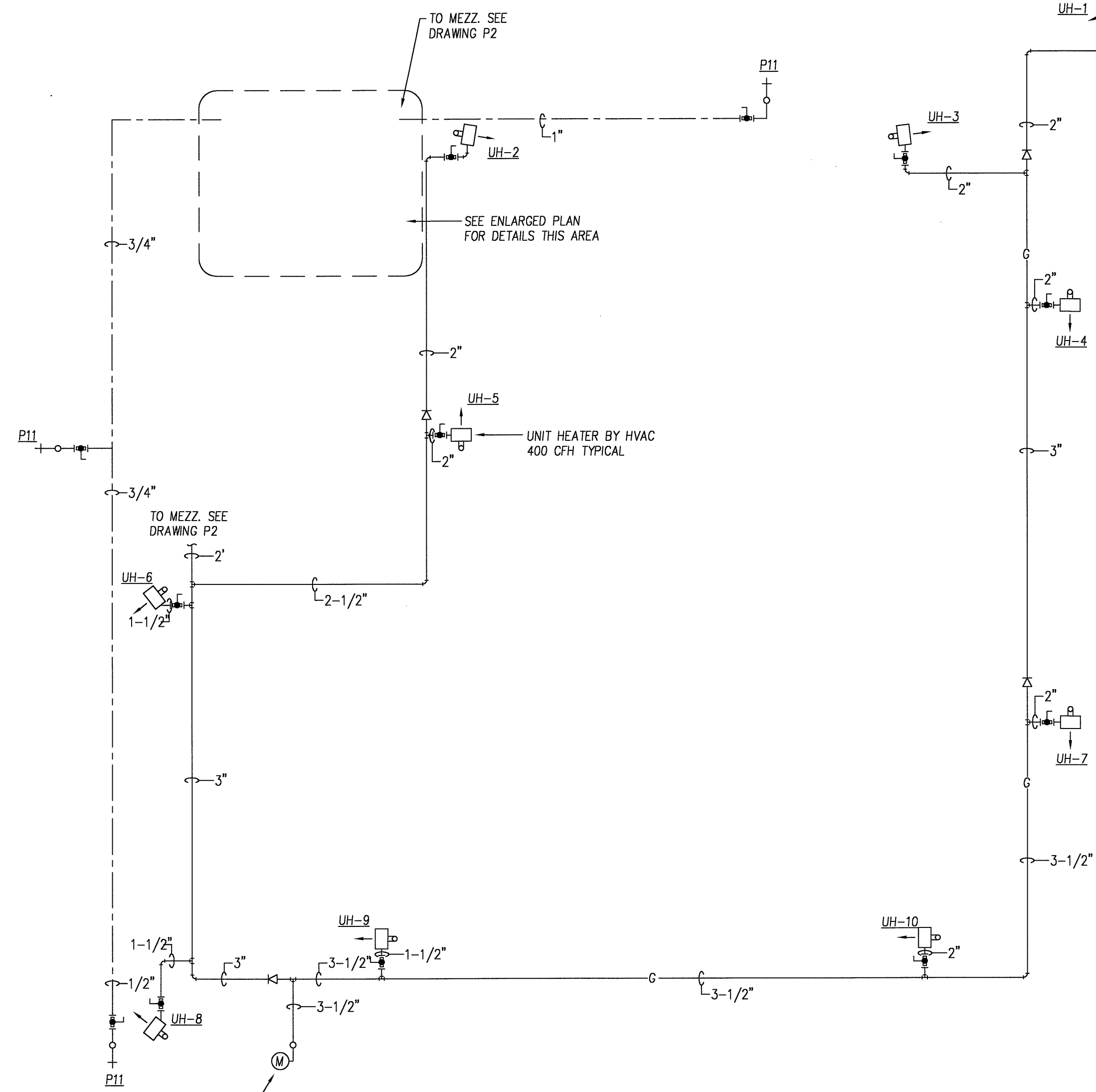
WAREHOUSE PHASE I PLAN 1/16" = 1' - 0"
