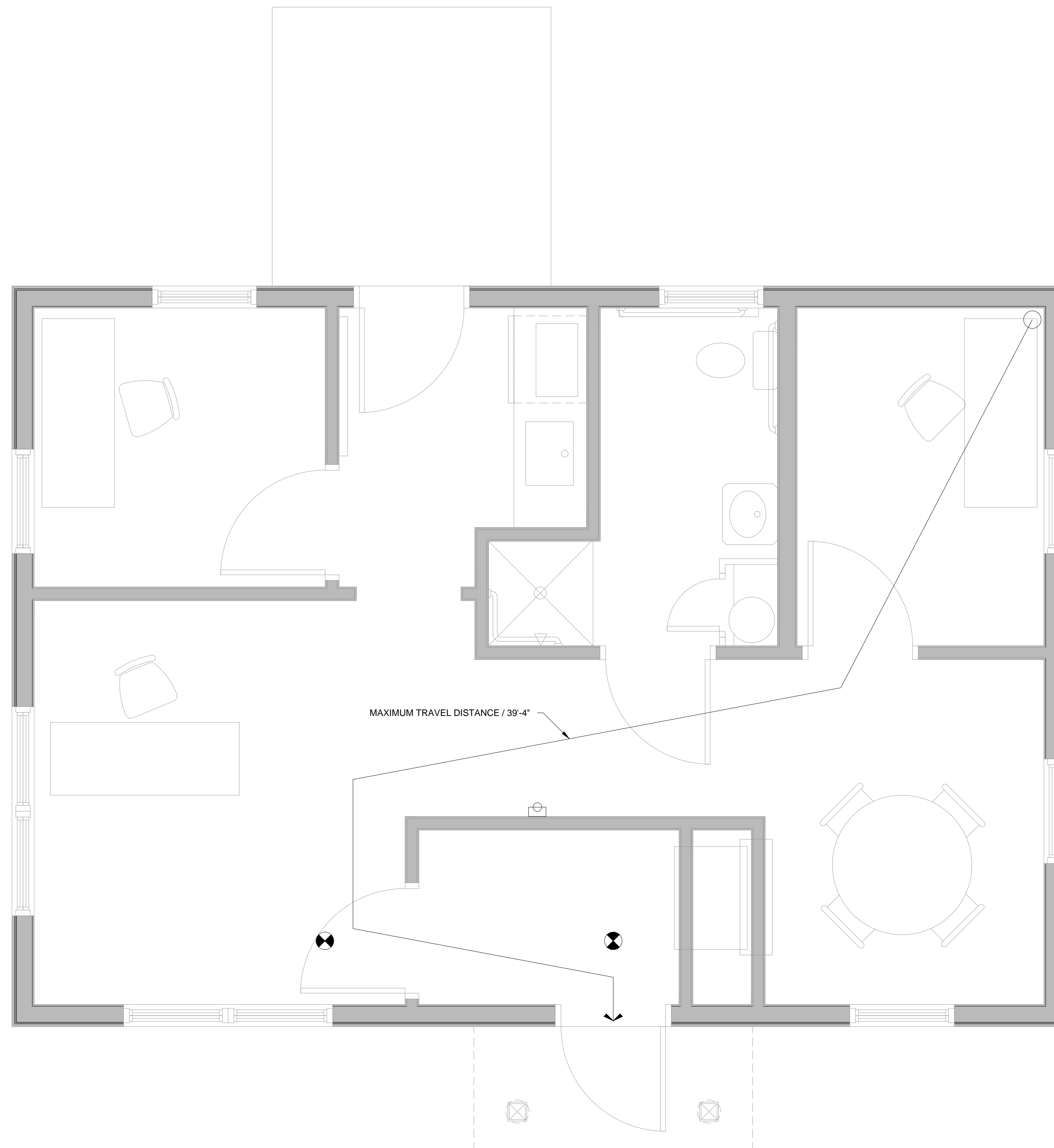
1 CODE REVIEW PLAN 1/2" = 1'-0"
