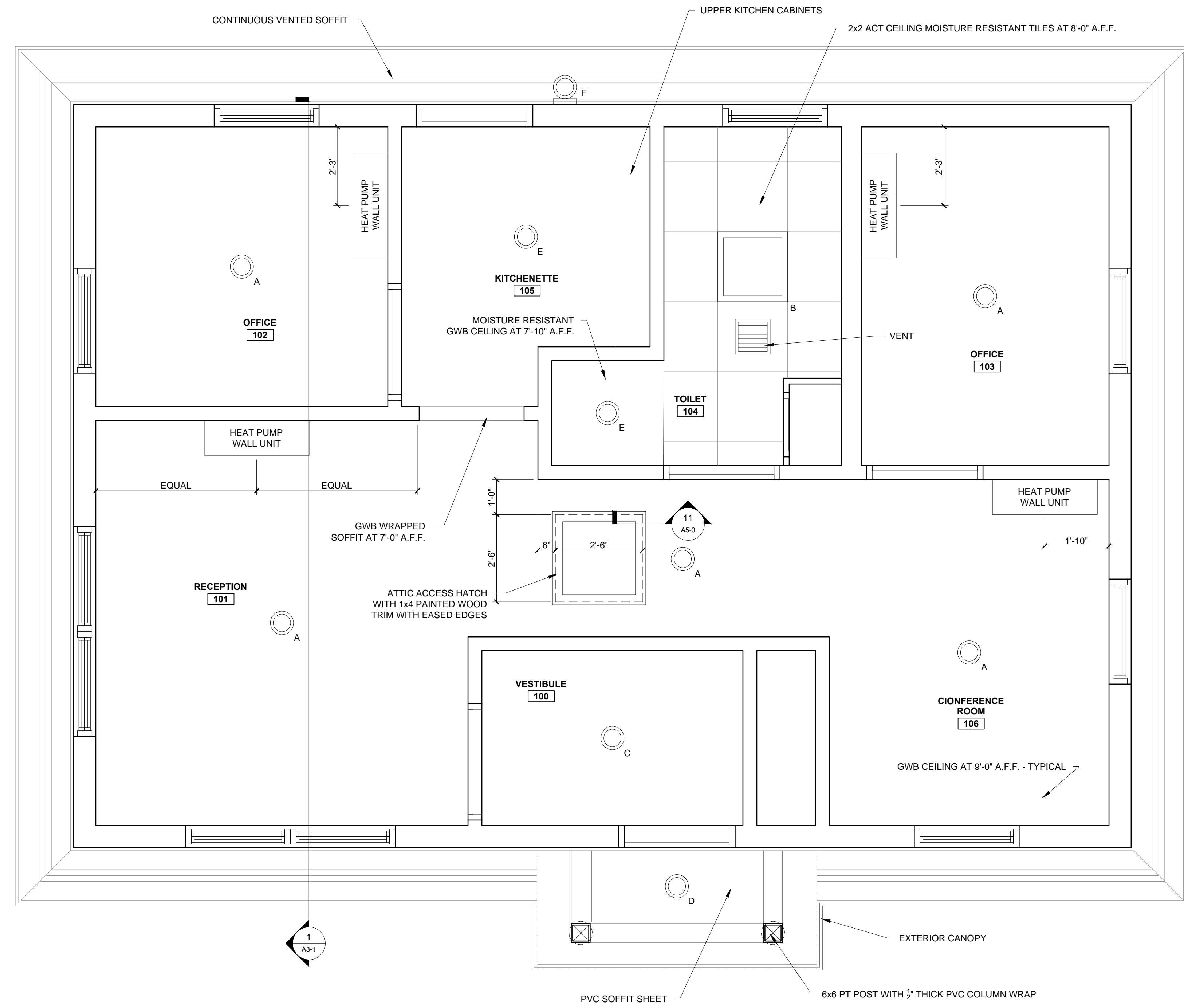
1 REFLECTED CEILING PLAN 1/2" = 1'-0"
