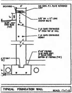
TYPICAL FOUNDATION WALL SCALE: 1"=1'-0"
