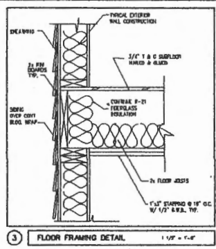
FLOOR FRAMING DETAIL SCALE: 1"=1'-0"
