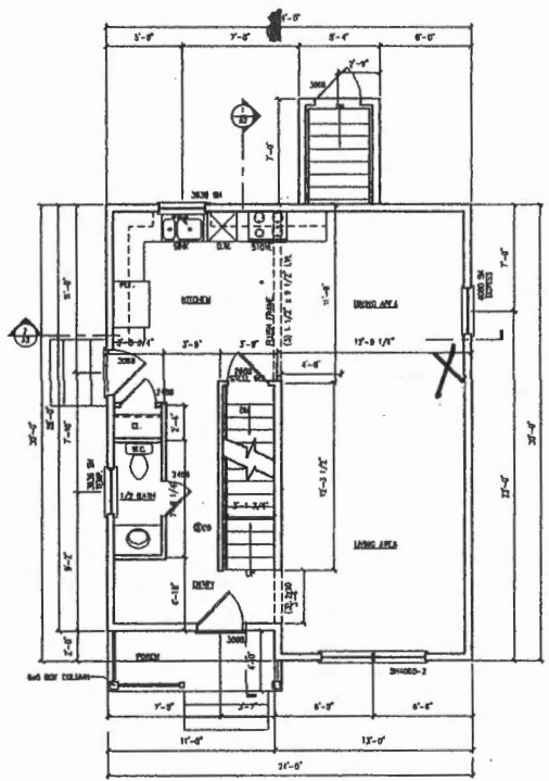
FIRST FLOOR PLAN SCALE: 1/4"=1'-0"
