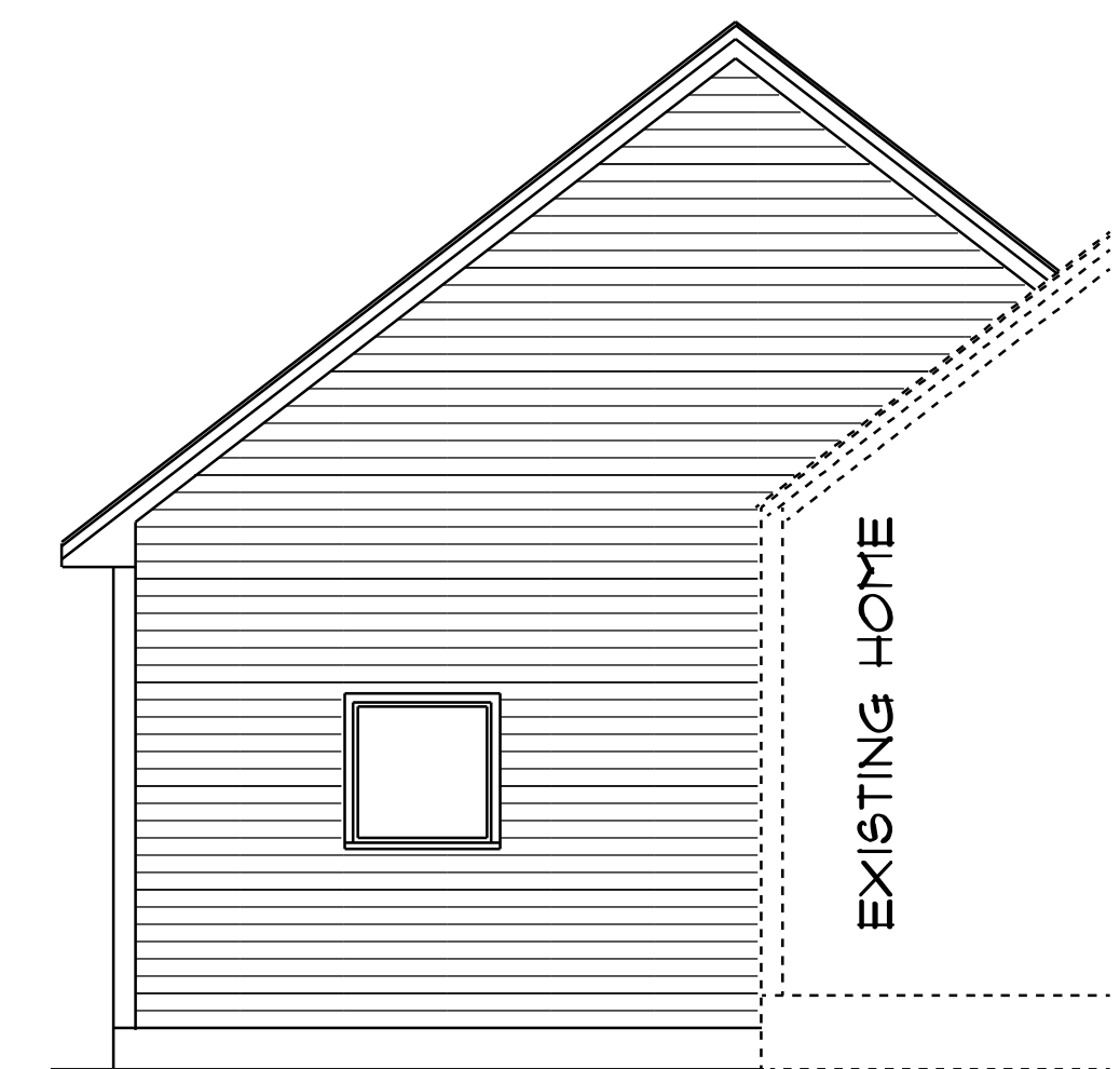
LEFT ELEVATION
