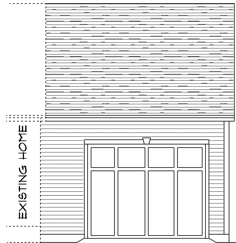
FRONT ELEVATION
