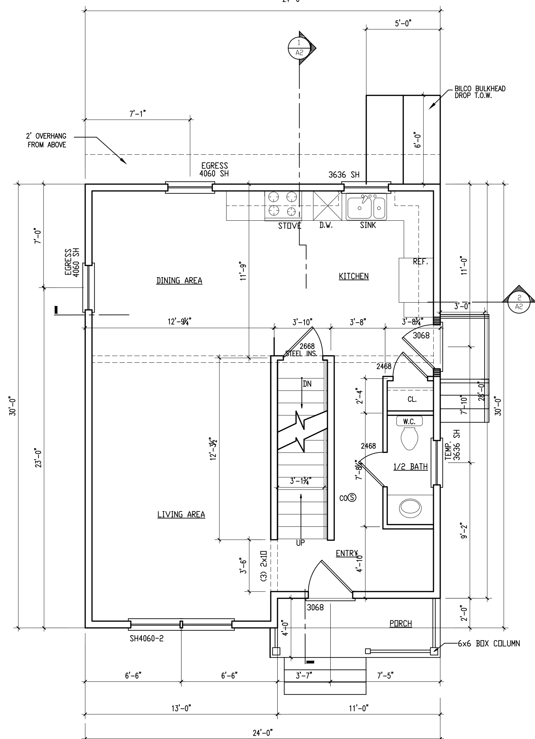
FIRST FLOOR PLAN SCALE: 1/4"=1'-0" 698 S.F.
