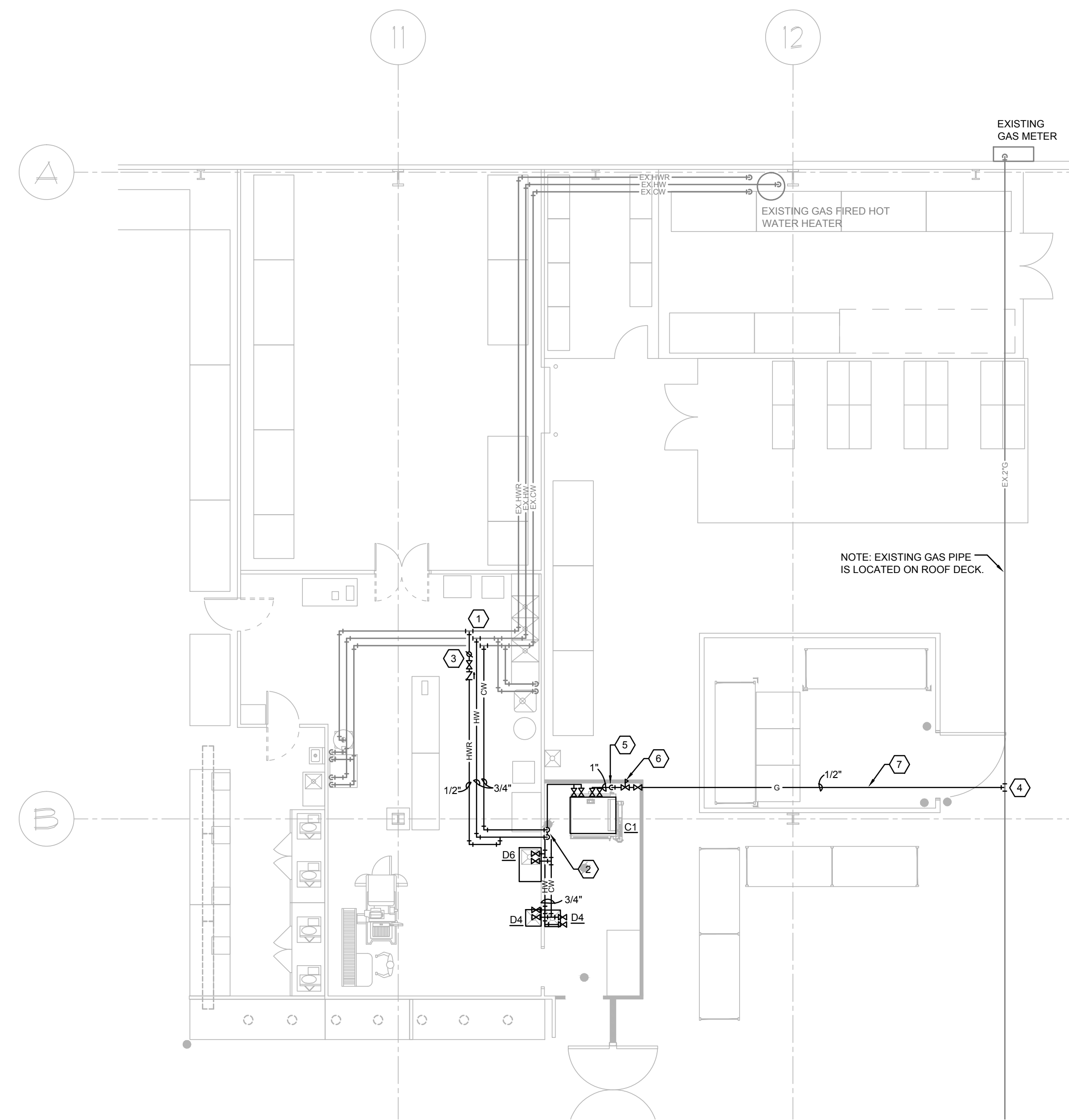
2 PLUMBING DOMESTIC WATER AND NATURAL GAS PLAN P100 SCALE: 1/8" = 1'-0"
