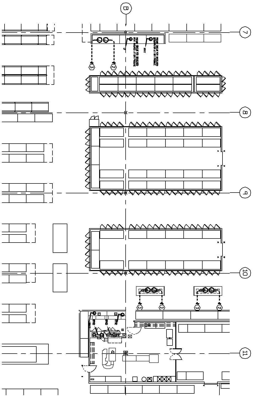
POWER PLAN SCALE 3/8" = 1'-0"
