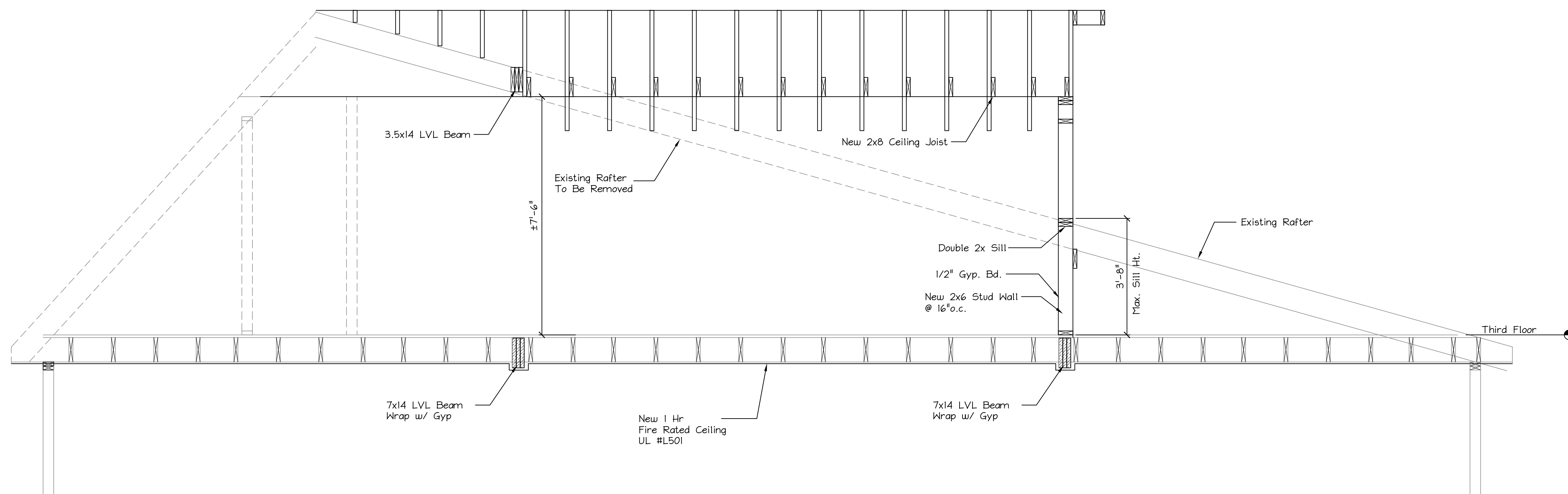
SECTION 5 @ NEW 3RD FLOOR DORMER B Scale: 1/2" = 1'-0"
