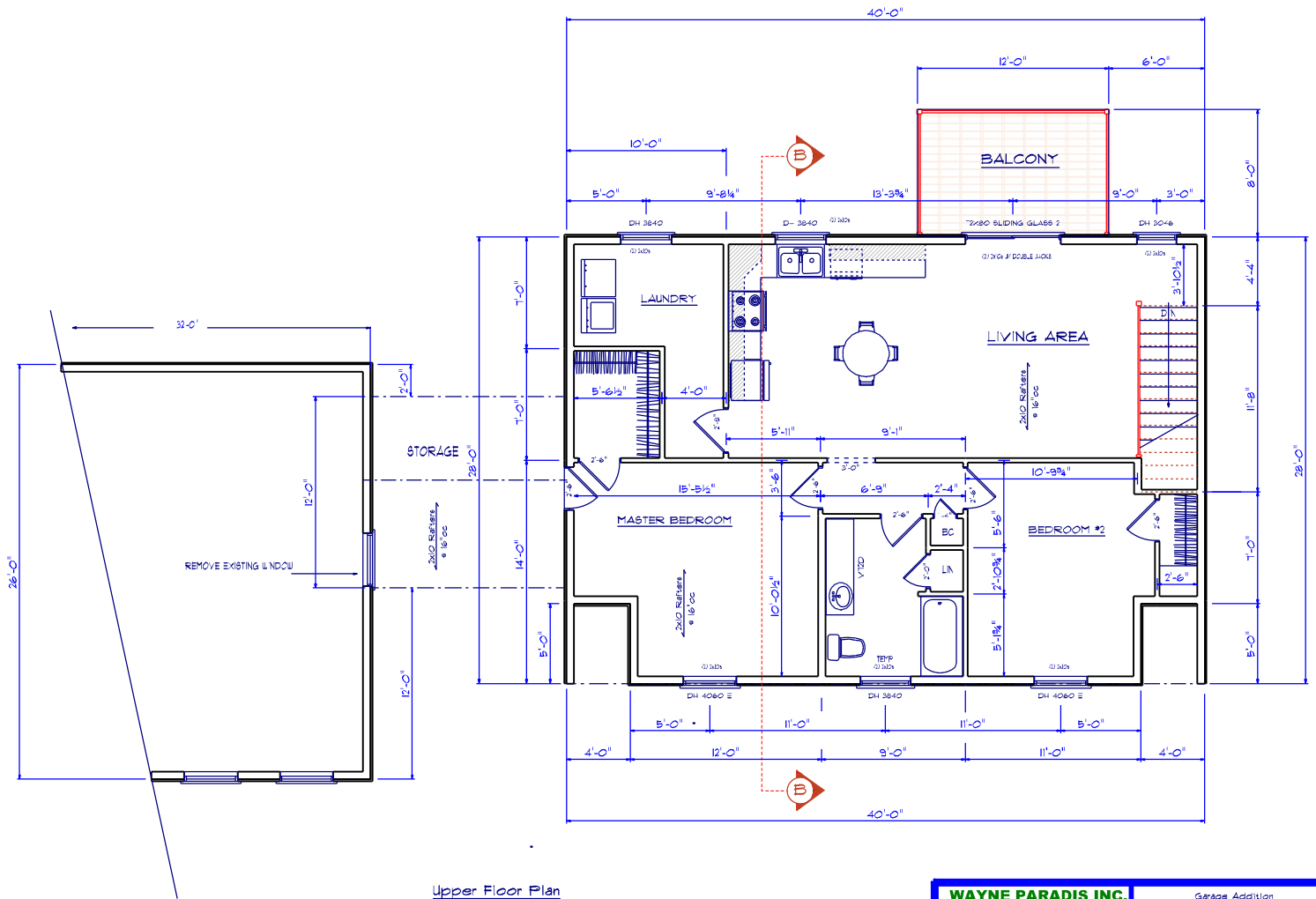
Upper Floor Plan 1/4" = 1'-0"
