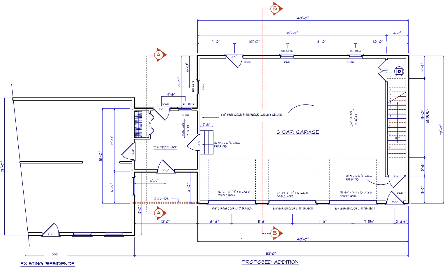
Lower Floor Plan 1/4" = 1'-0"
