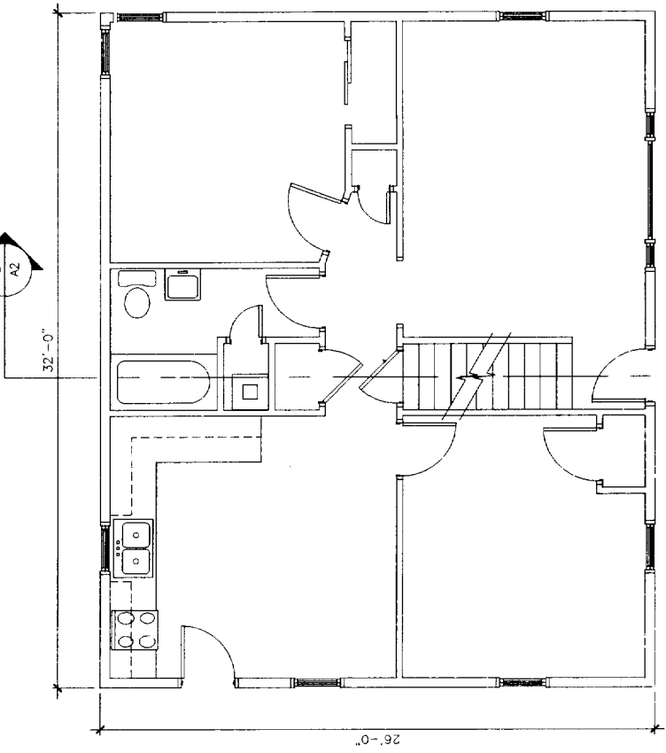
1 EXIST. FIRST FLOOR SCALE: 1/4"=1'-0"
