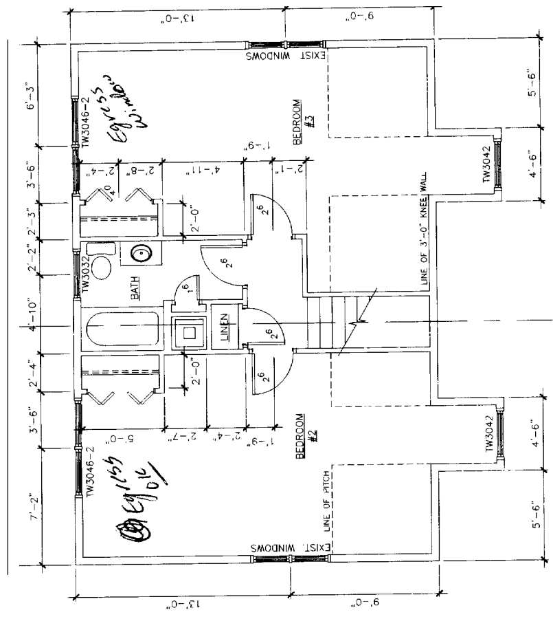
2 SECOND FLOOR PLAN SCALE: 1/4"=1'-0"
