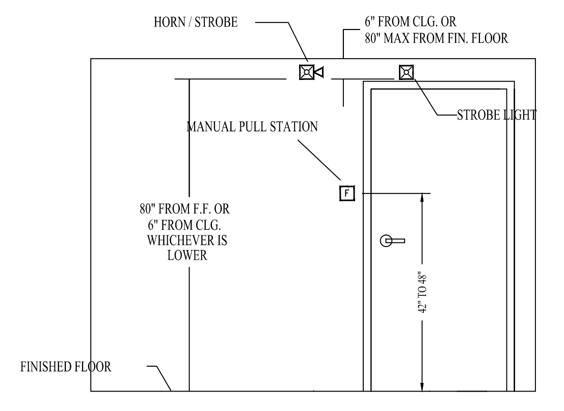
DEVICE ELEVATION DETAIL NOT TO SCALE
