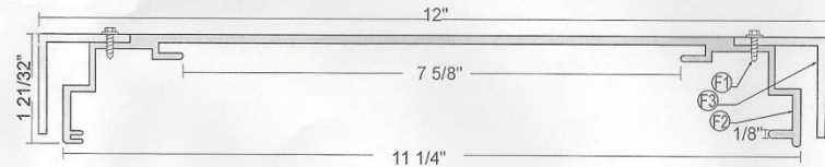
12" wide TSA extrusion with 1 1/2" Retainer
