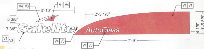
Graphics Layout
