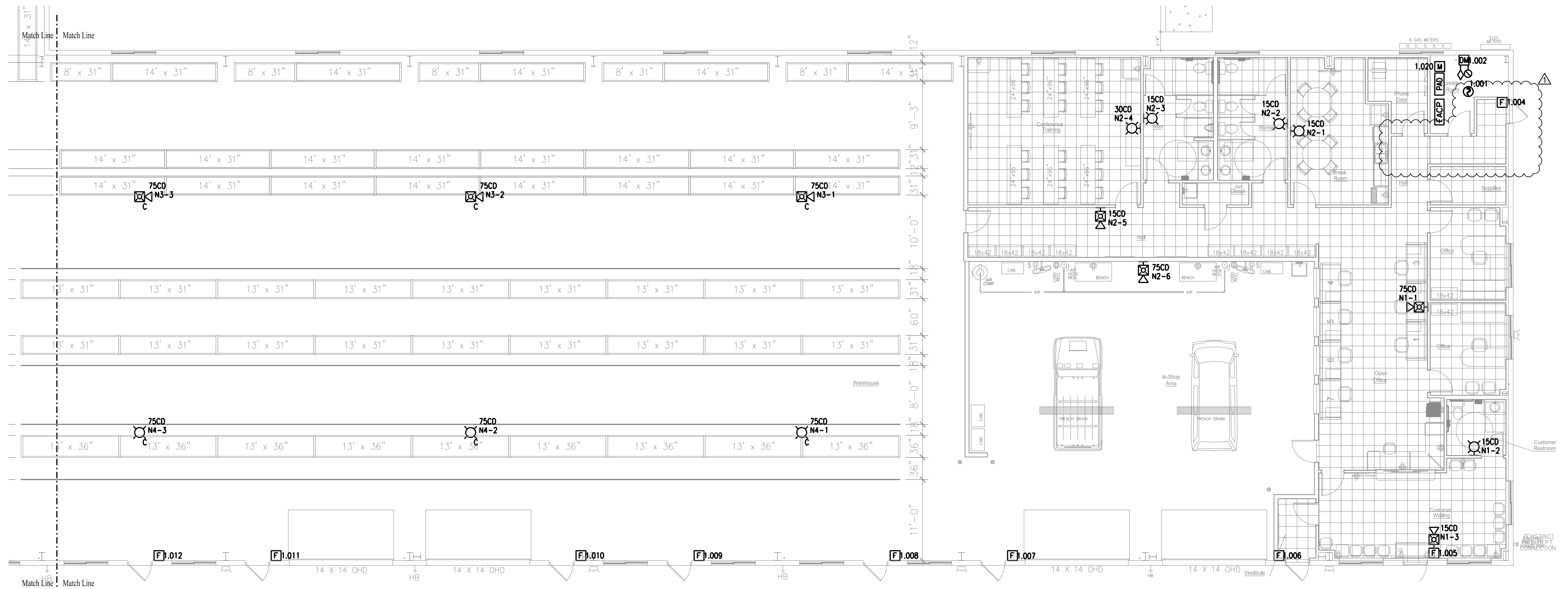
FIRE ALARM SYSTEM LAYOUT - WAREHOUSE & OFFICE AREA SCALE: 1/8" = 1'
