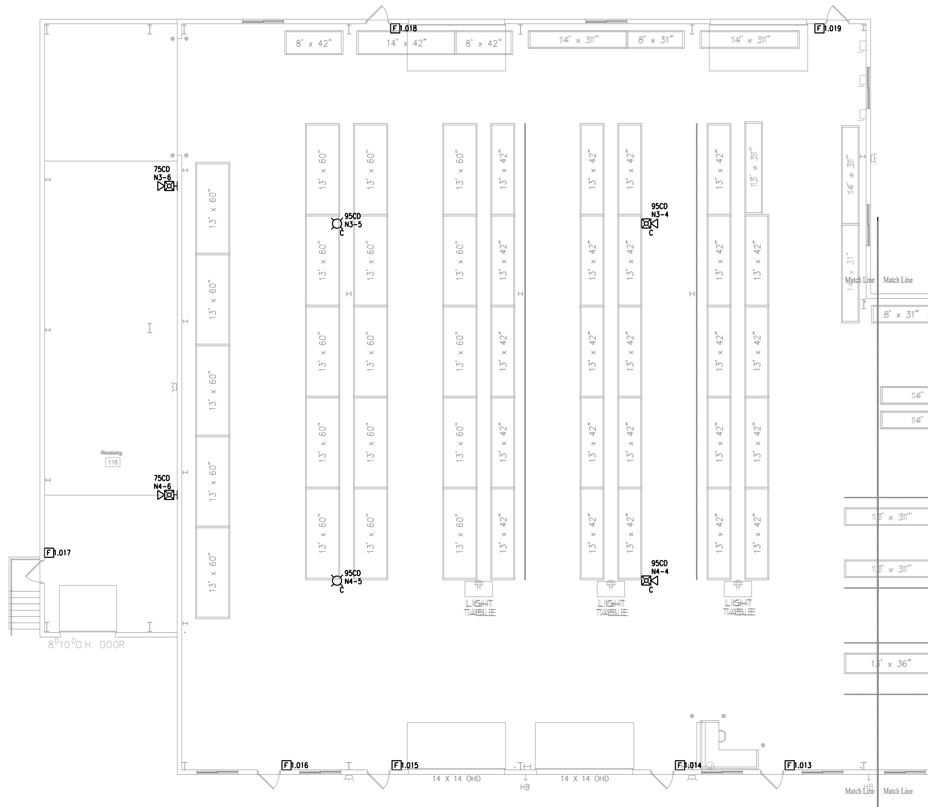
FIRE ALARM SYSTEM LAYOUT - WAREHOUSE AREA SCALE: 1/8" = 1'
