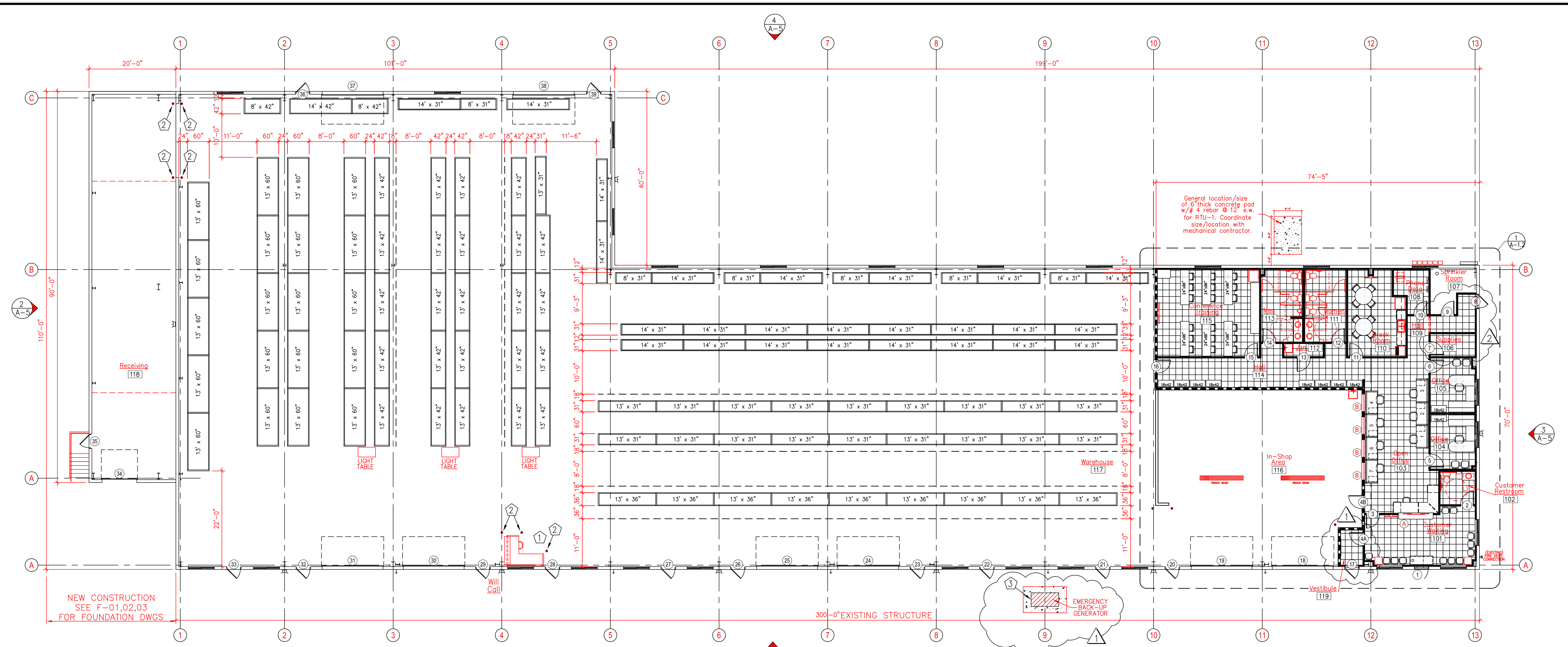
1 FLOOR PLAN SCALE - 3/32"=1'-0"
