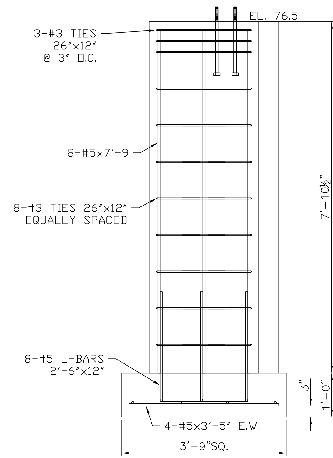
A-2 SECTION & DETAIL
