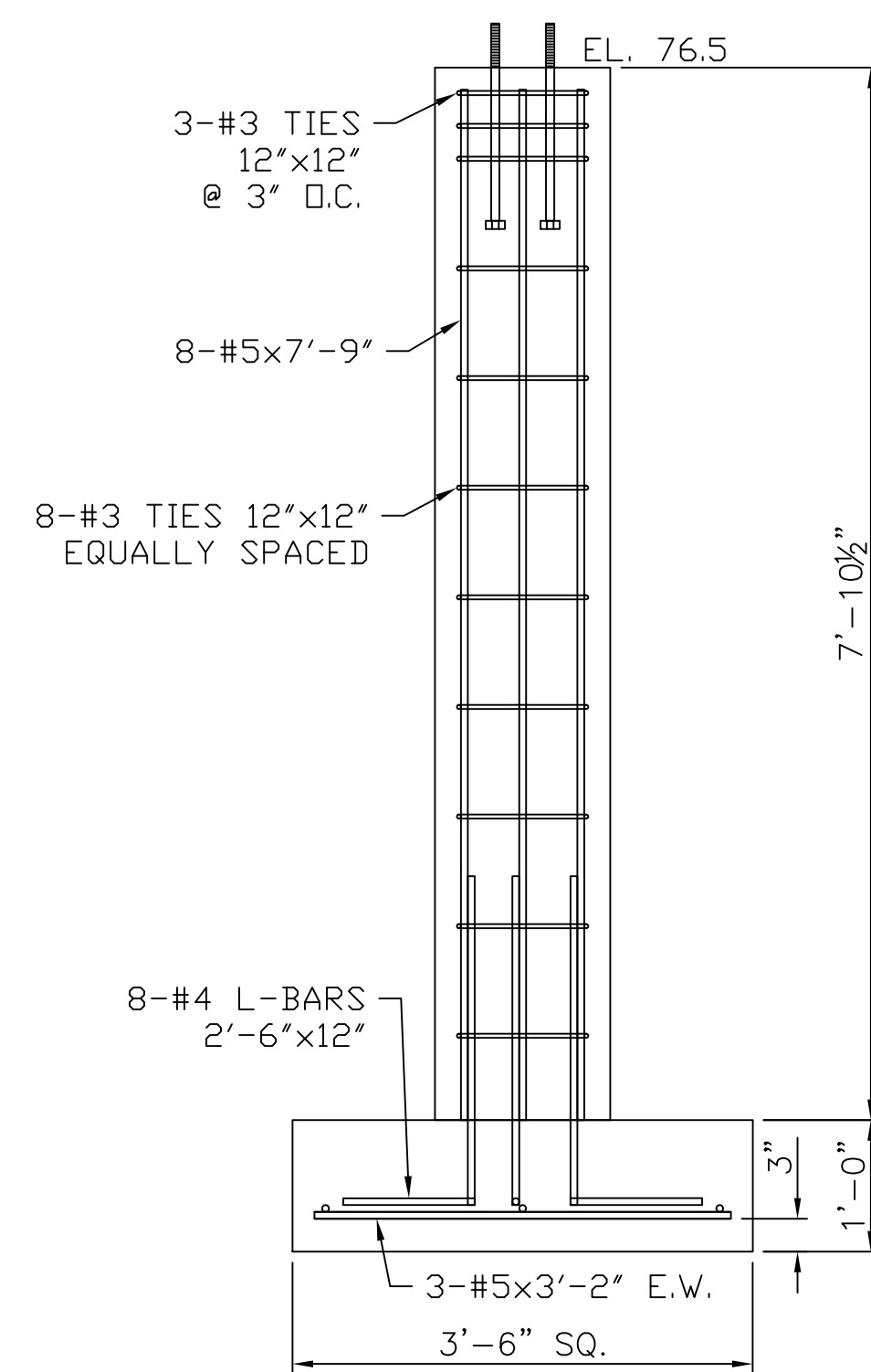
A-1 SECTION & DETAIL
