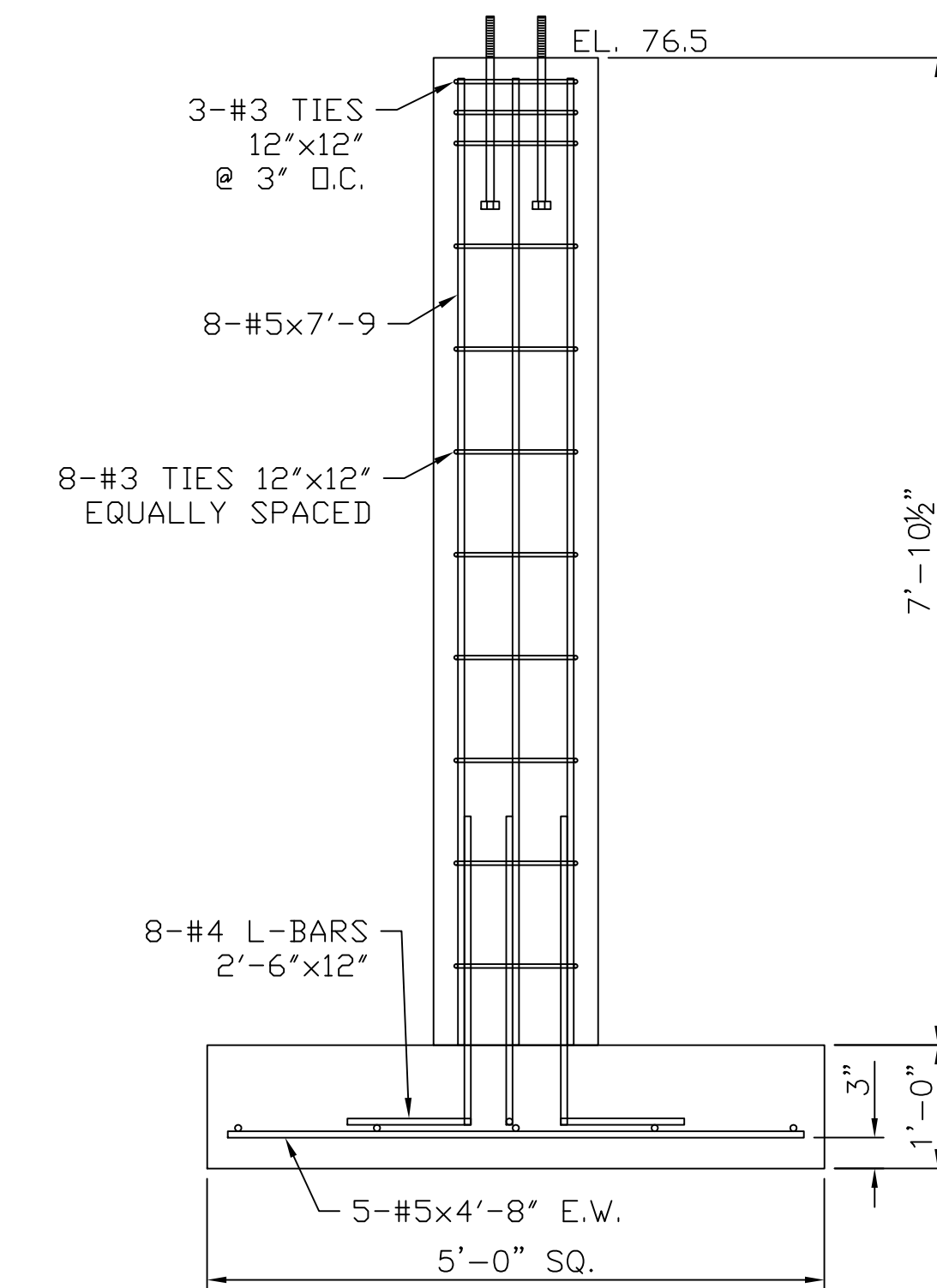
B,C,D-1 SECTION & DETAIL
