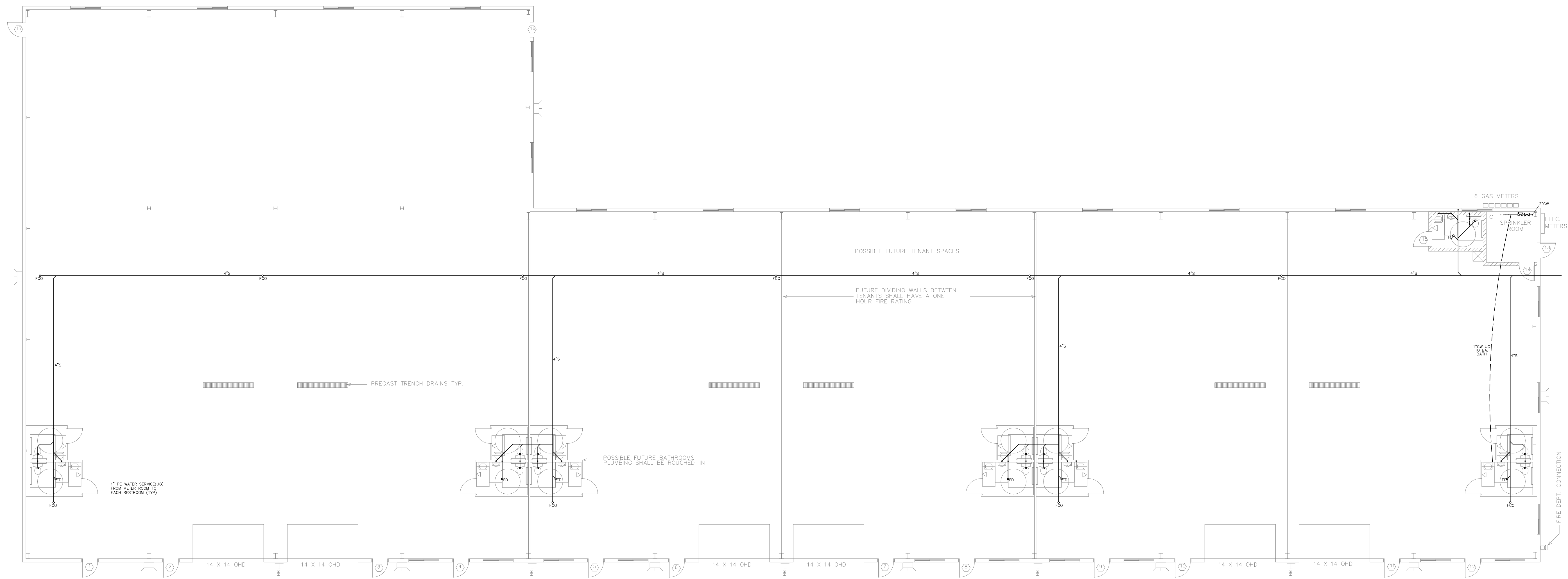
PLUMBING PLAN SCALE: 3/32" = 1'-0"
