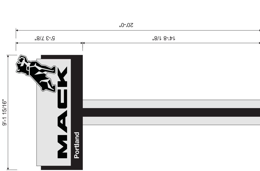
NMP-40 Pylon Sign Scale 1/4" = 1'-0"
