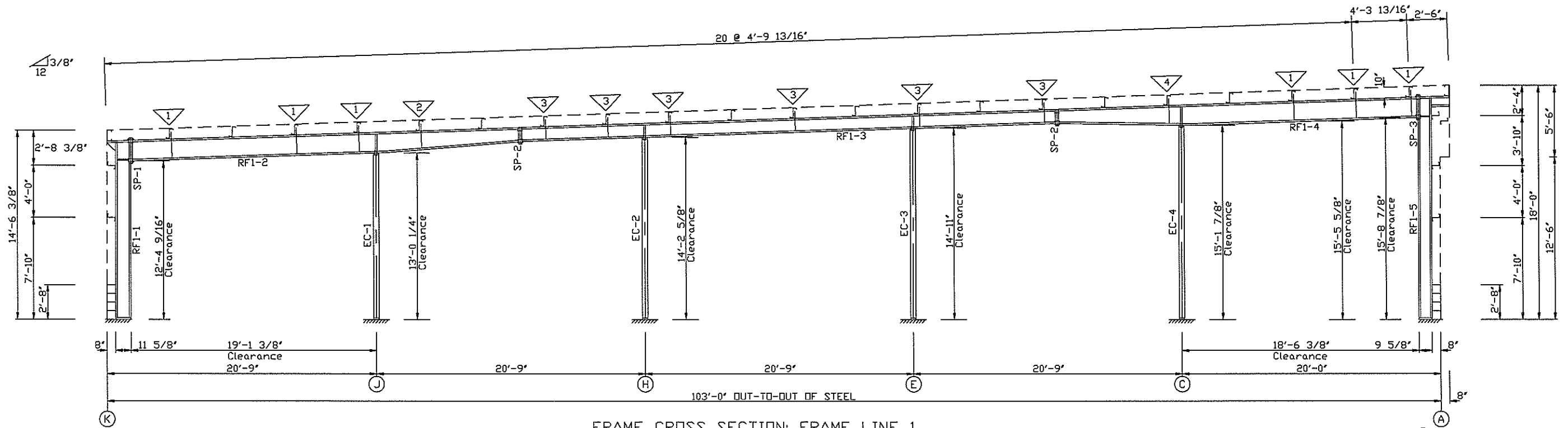
FRAME CROSS SECTION: FRAME LINE 1
