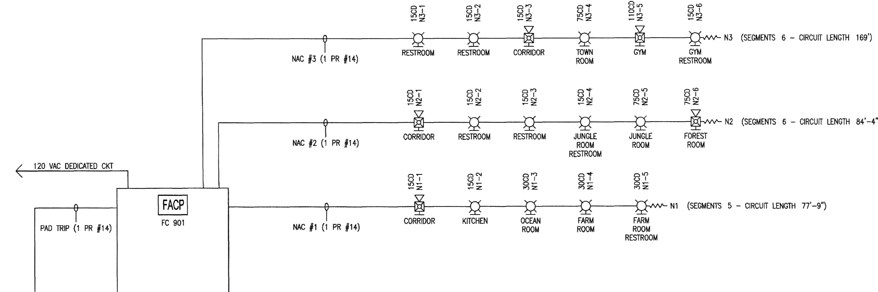
FIRE ALARM RISER DIAGRAM SCALE NTS
