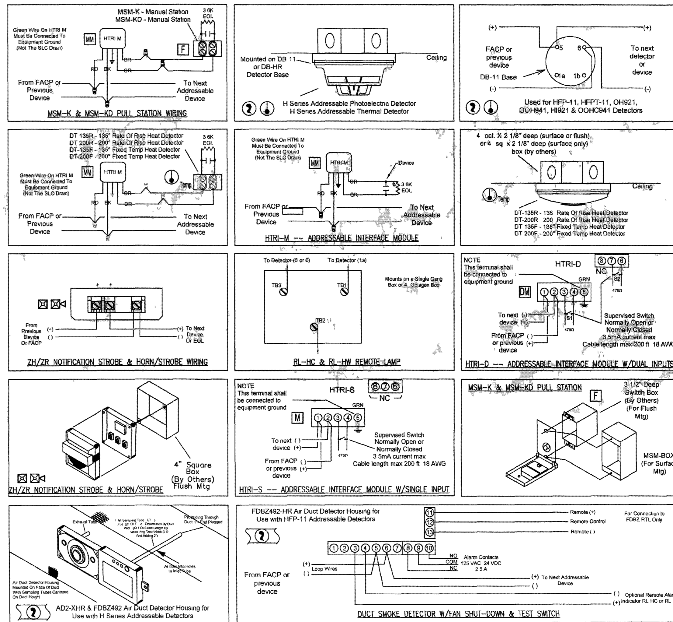
DEVICE WIRING DETAIL SCALE NTS
