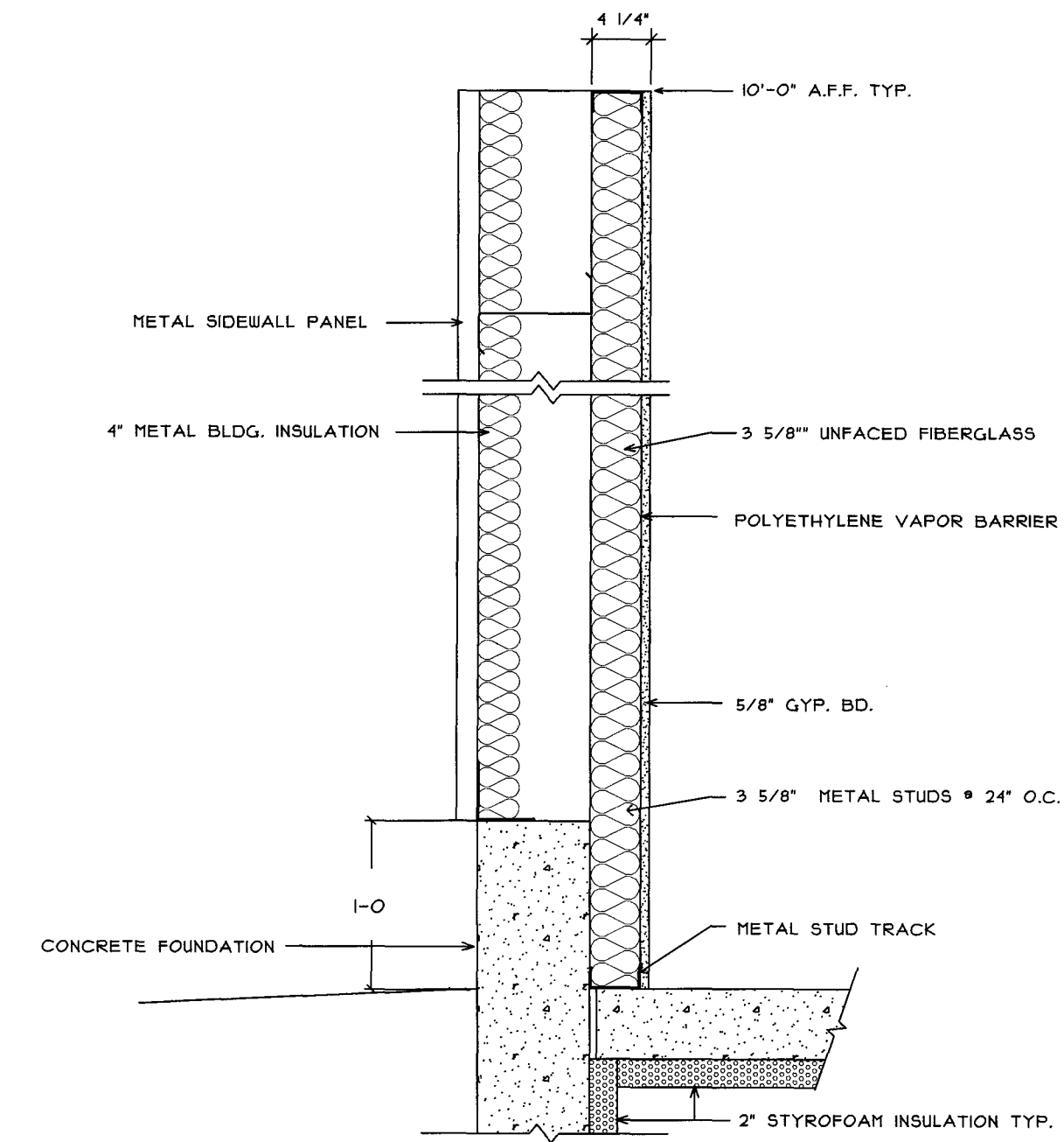
5 EXTERIOR WALL @ METAL SIDING SCALE: 1" = 1'-0"
