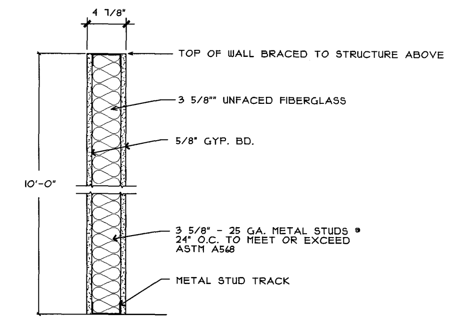
1 INTERIOR PARTITION TYP. U.N.O. SCALE: 1" = 1'-0"
