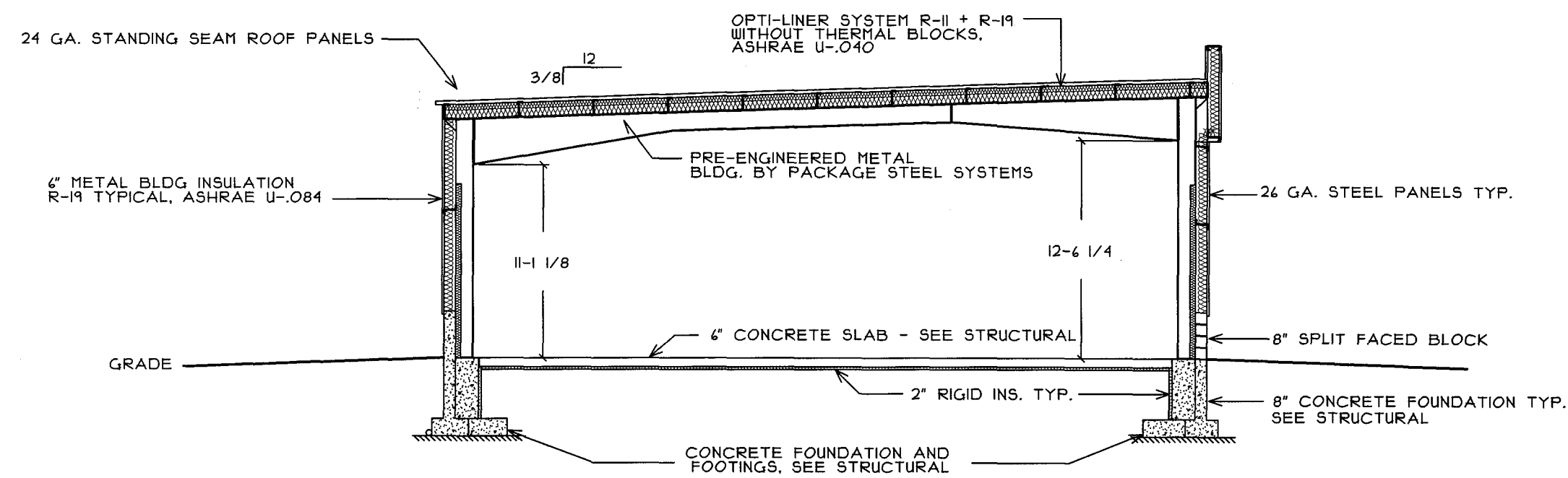
BUILDING SECTION SCALE: 1/8" = 1'-0"
