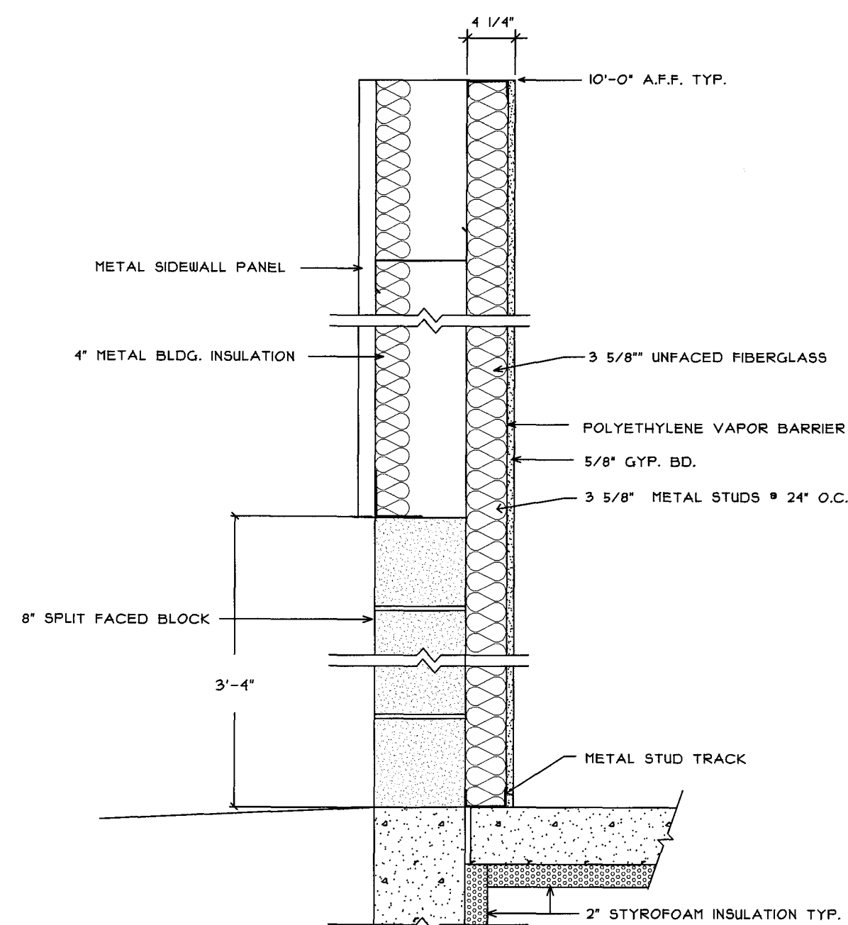
4 EXTERIOR WALL @ BLOCK WALL SCALE: 1" = 1'-0"
