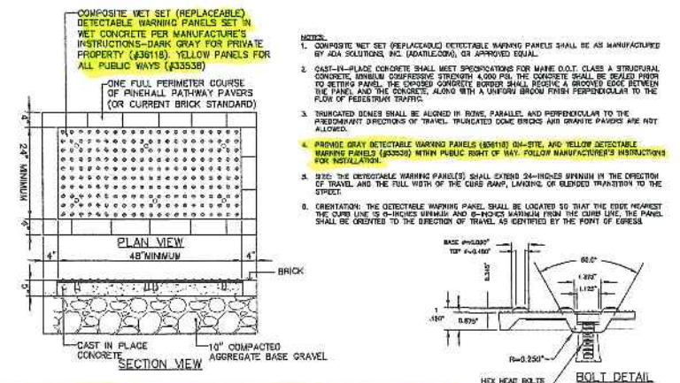
15 SIDEWALK RAMP DETECTABLE WARNING TILE L5 NOT TO SCALE
