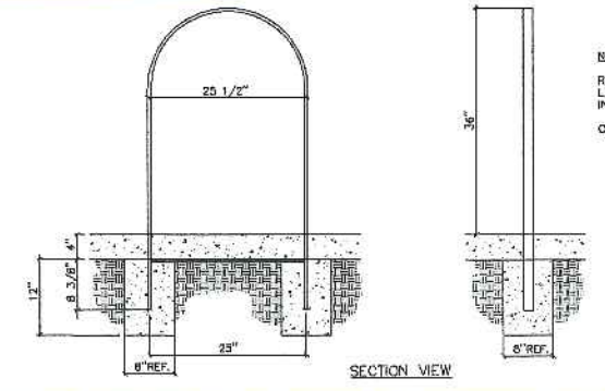
13 WABASH VALLEY 'BIKE LOOPS' PLASTISOL COATED- BIKE RACK L5 NOT TO SCALE
