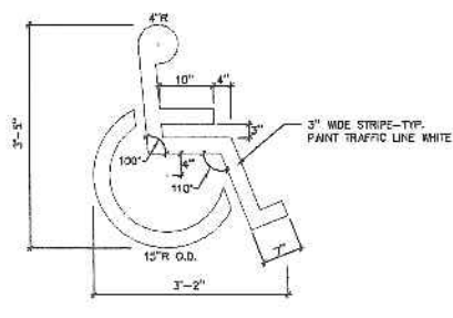
11 ACCESSIBLE SPACE MARKINGS L5 NOT TO SCALE
