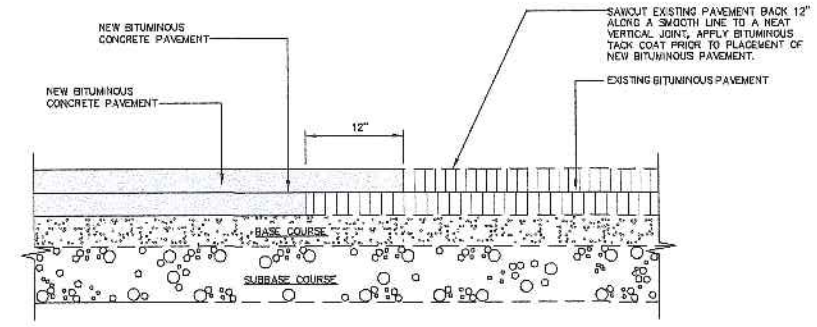
9 PAVEMENT SAWCUT DETAIL L5 NOT TO SCALE
