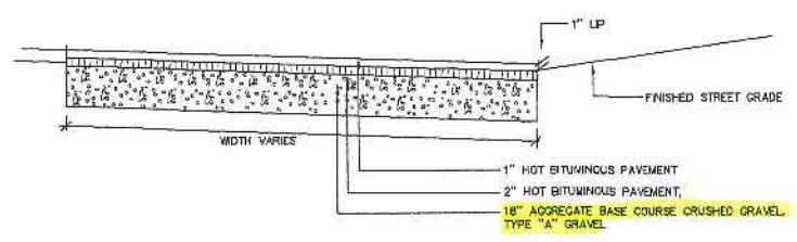
5 BITUMINOUS DRIVEWAY APRON L5 NOT TO SCALE
