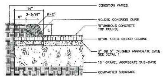
7 SLIPFORM CONCRETE CURB-DRIVEWAY L5 NOT TO SCALE
