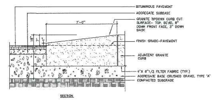
8 GRANITE TIP-DOWN CURB - CITY RIGHT OF WAY L5 NOT TO SCALE
