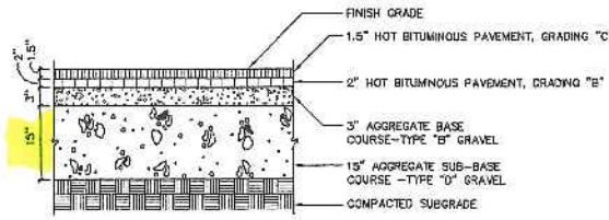
1 BITUMINOUS PAVEMENT- LOCAL STREET - CITY OF PORTLAND STANDARD L5 NOT TO SCALE
