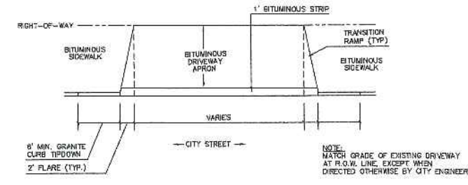
10 DRIVEWAY APRON LAYOUT L5 NOT TO SCALE
