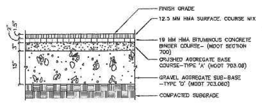
2 BITUMINOUS PAVEMENT- PARKING LOT L5 NOT TO SCALE
