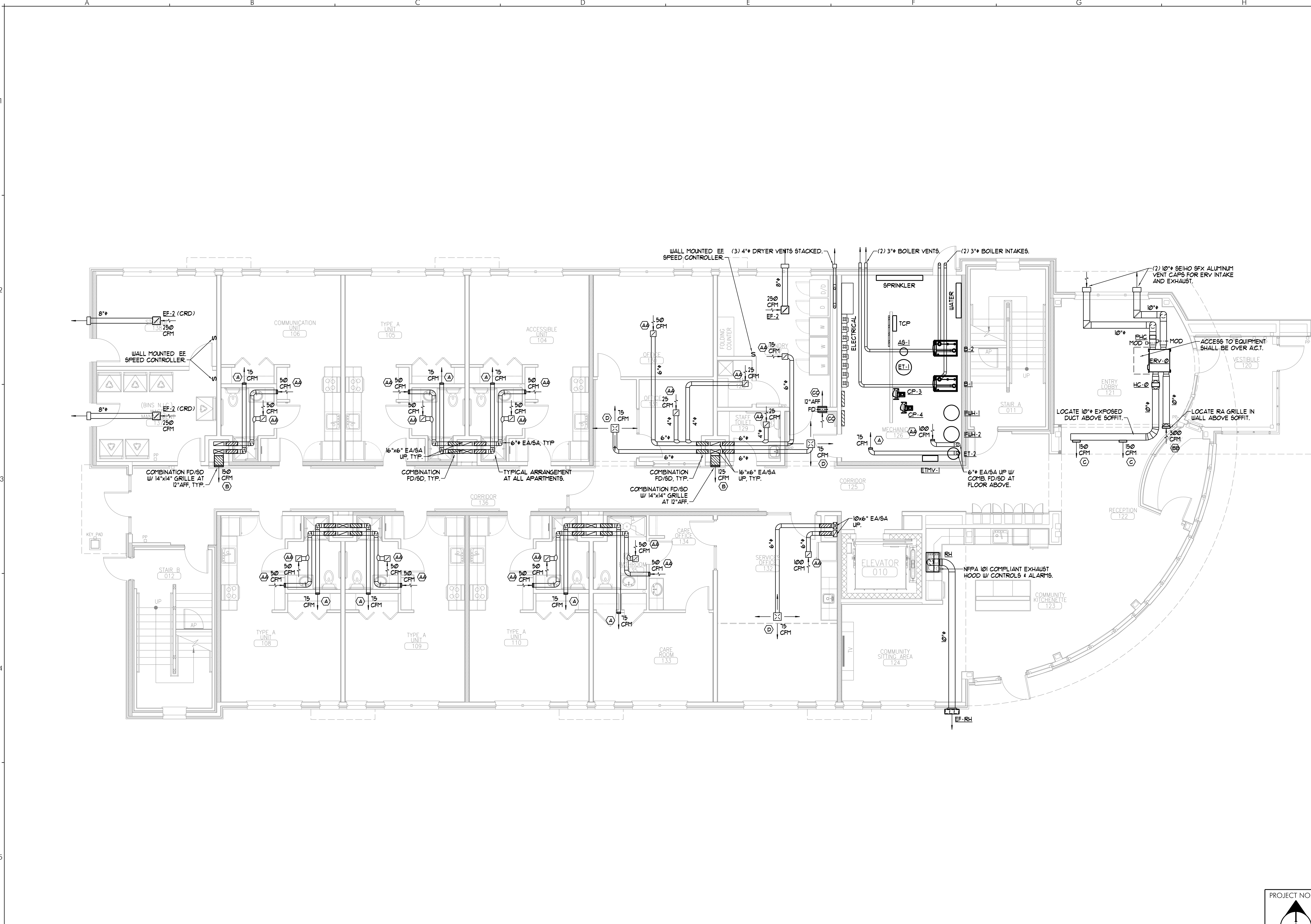
A5 FIRST FLOOR MECHANICAL DUCTWORK PLAN SCALE: 3/16" = 1'-0"
