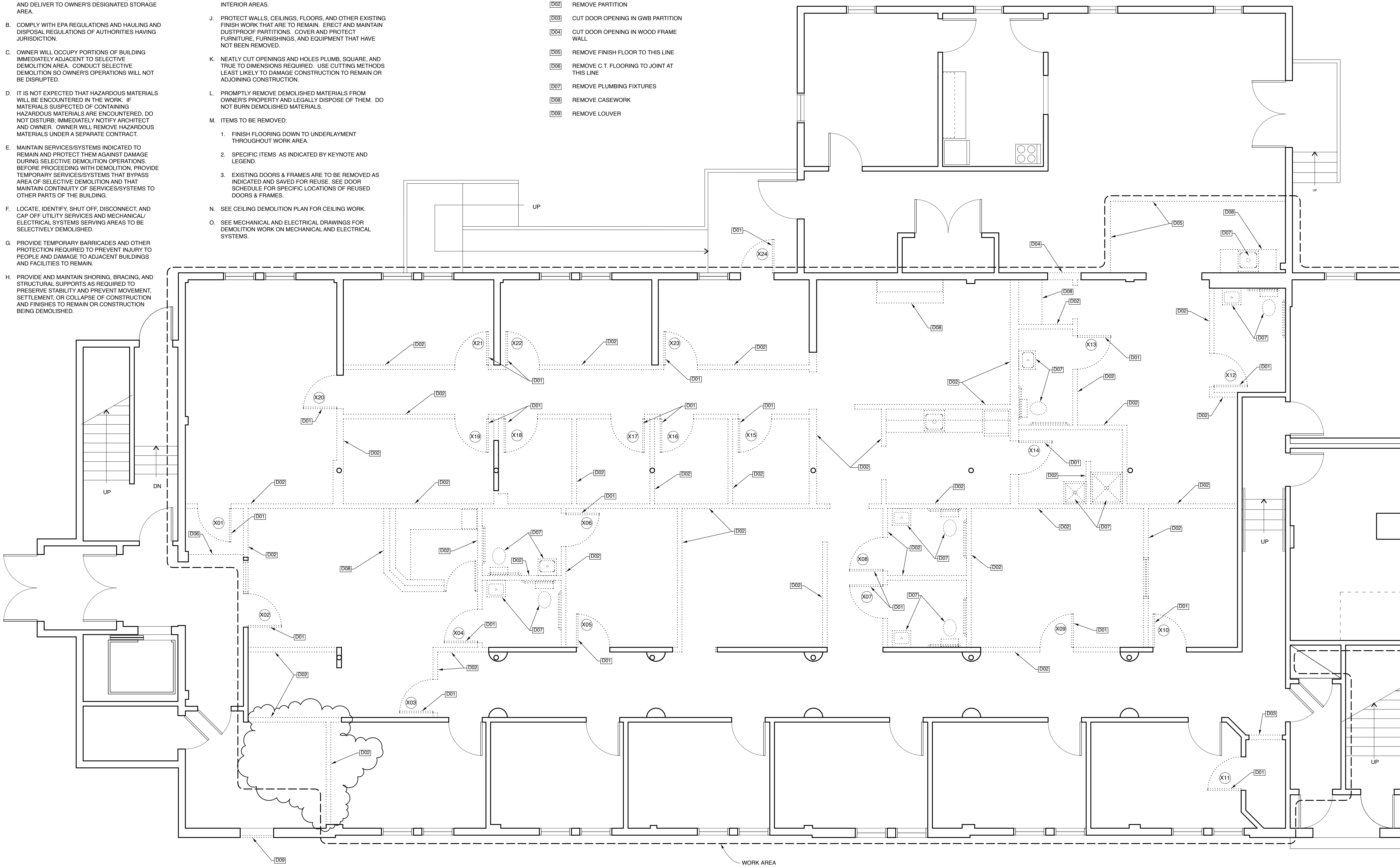
1 FIRST FLOOR DEMOLITION PLAN SCALE: 1/4" = 1'-0" 1' 2' 4' 8'
