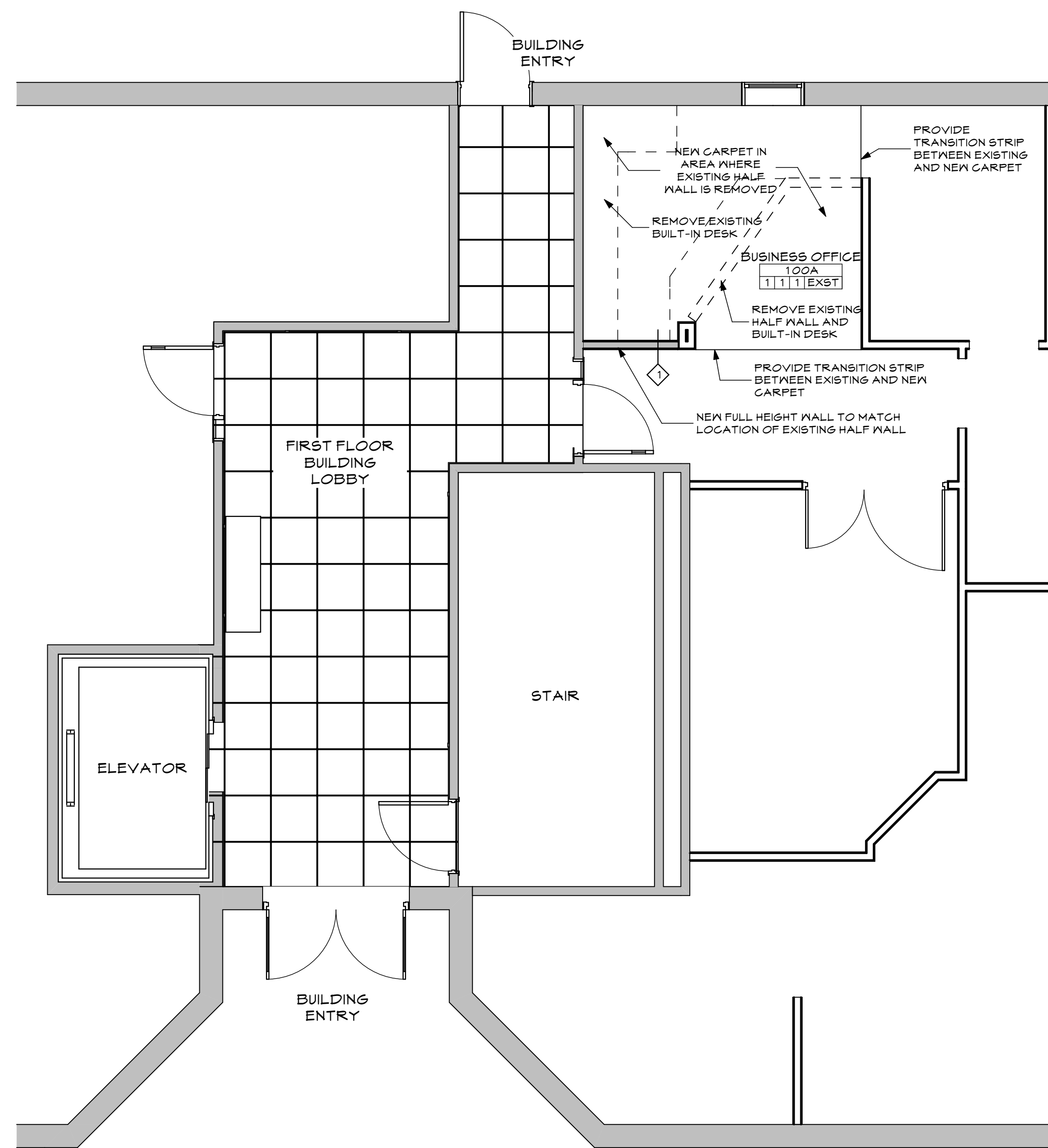
1 FIRST FLOOR PLAN A.5 SCALE: 1/4" = 1'-0"
