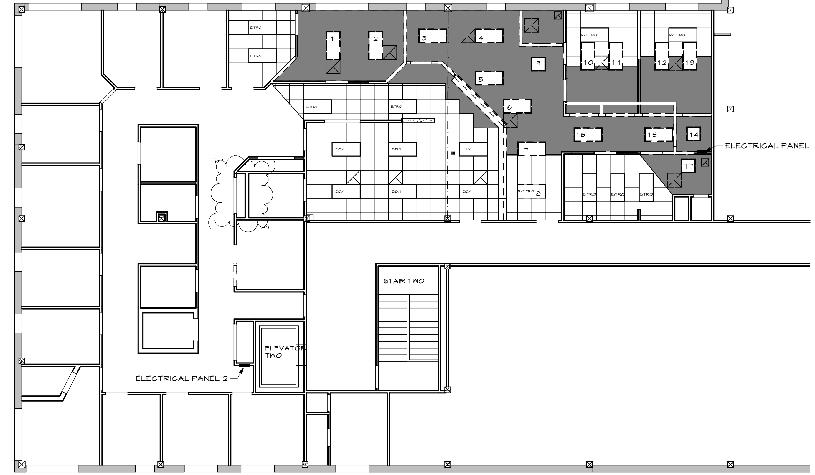
2 REFLECTED CEILING PLAN - DEMO SCALE: 1/8" = 1'-0"
