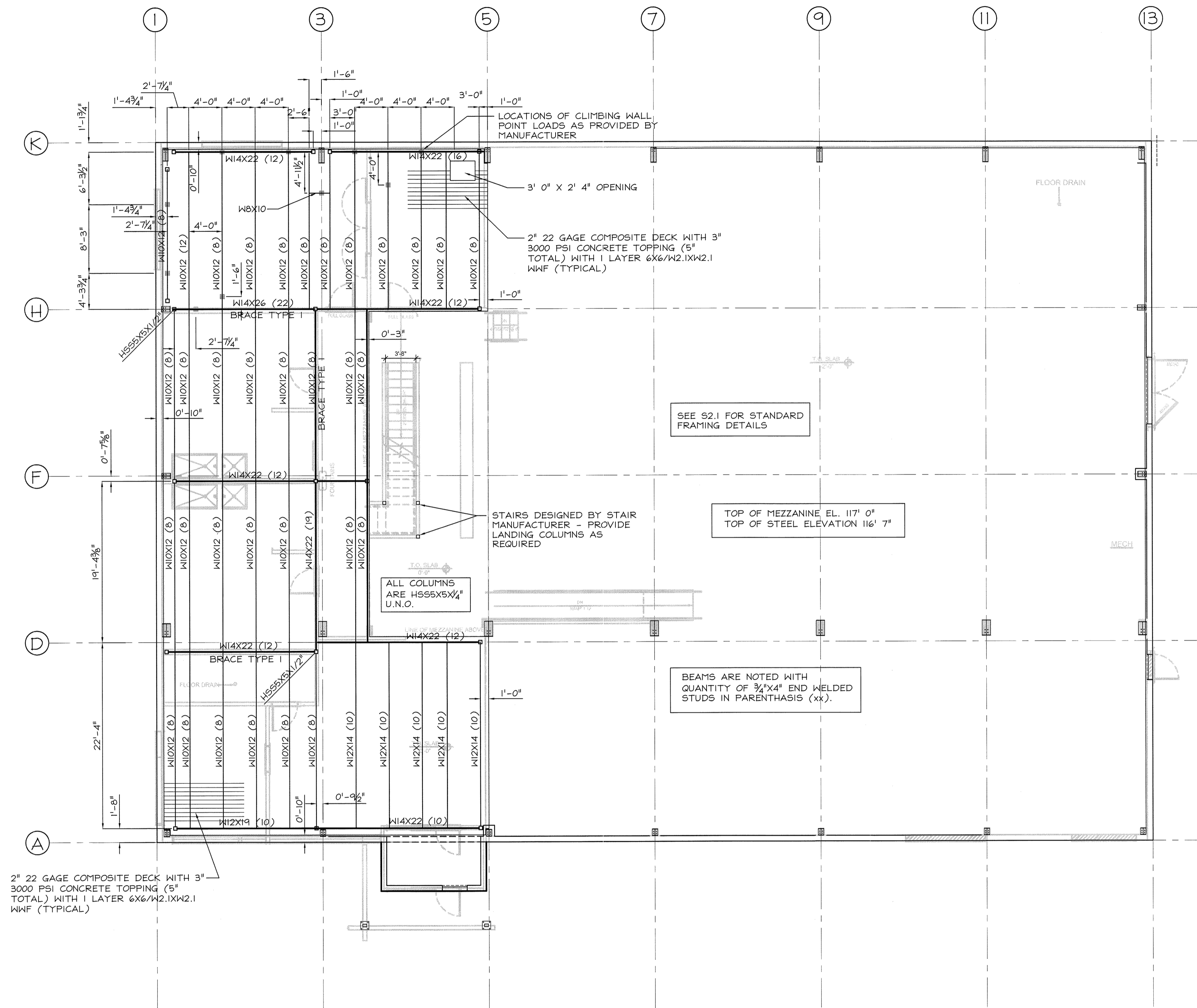
S2.0 MEZZANINE FRAMING PLAN Scale: 1/8" = 1'-0"
