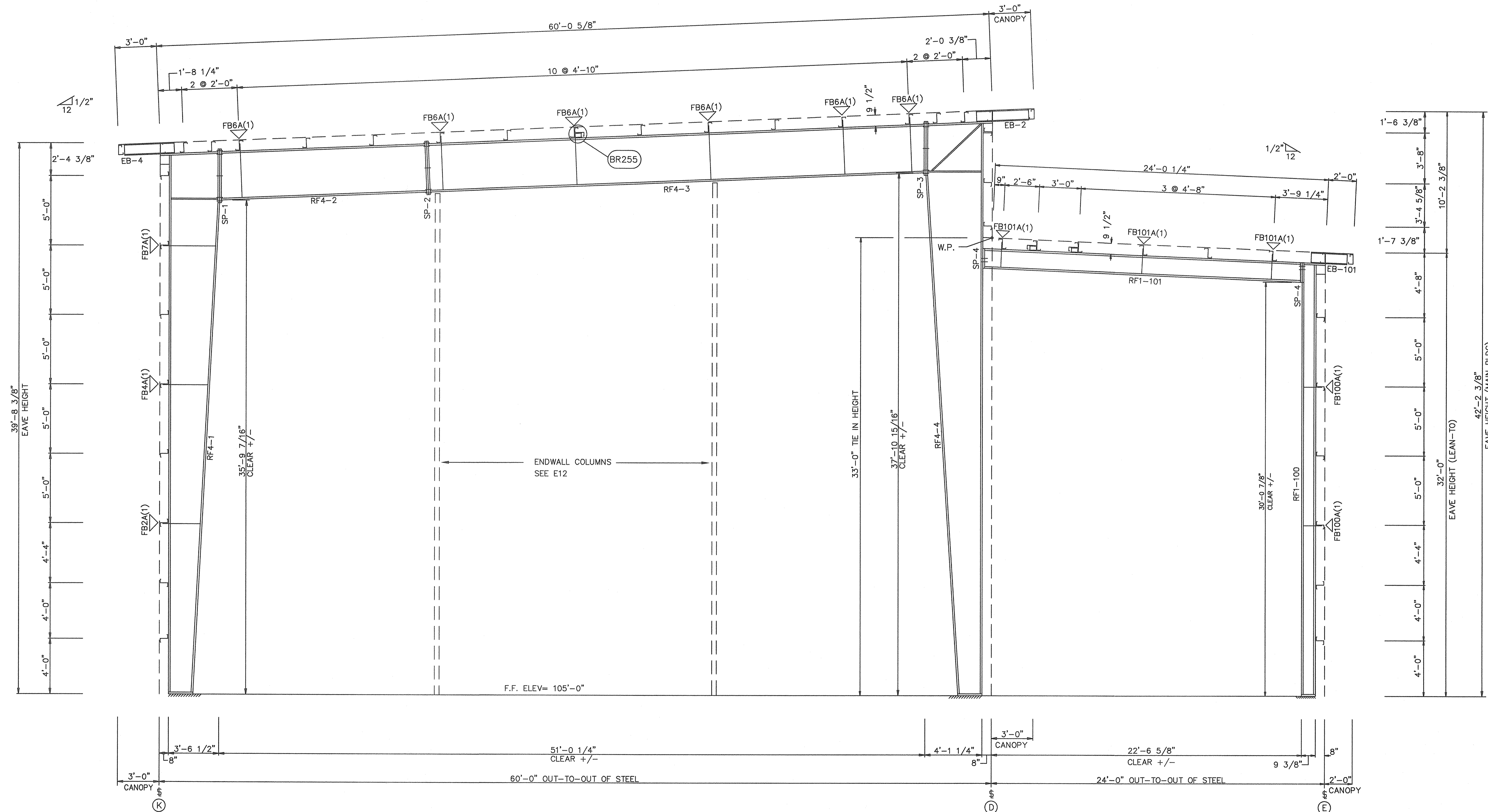
RIGID FRAME ELEVATION: FRAME LINE 13
