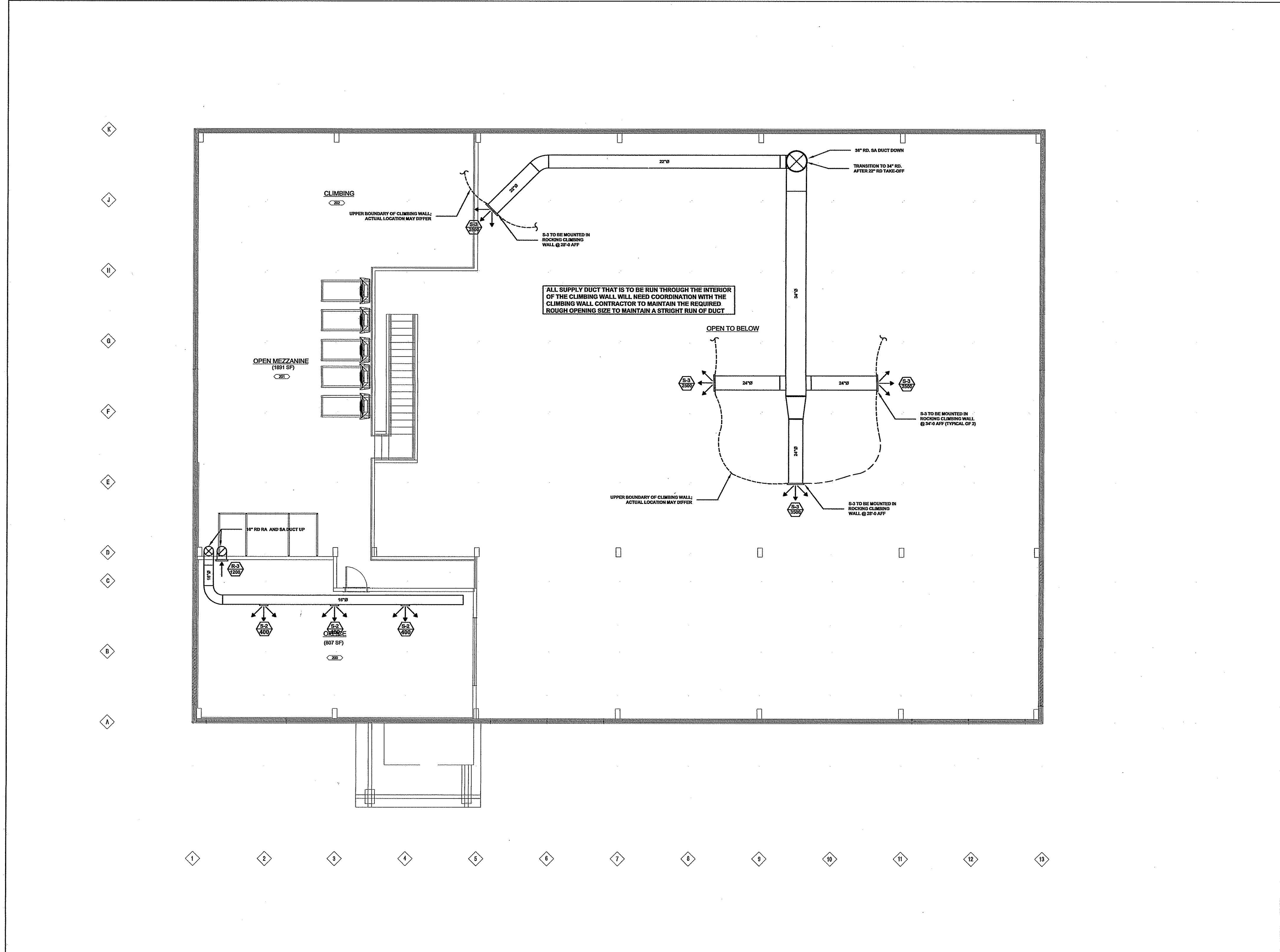
UPPER LEVEL HVAC PLAN SCALE: 1/8"=1'-0
