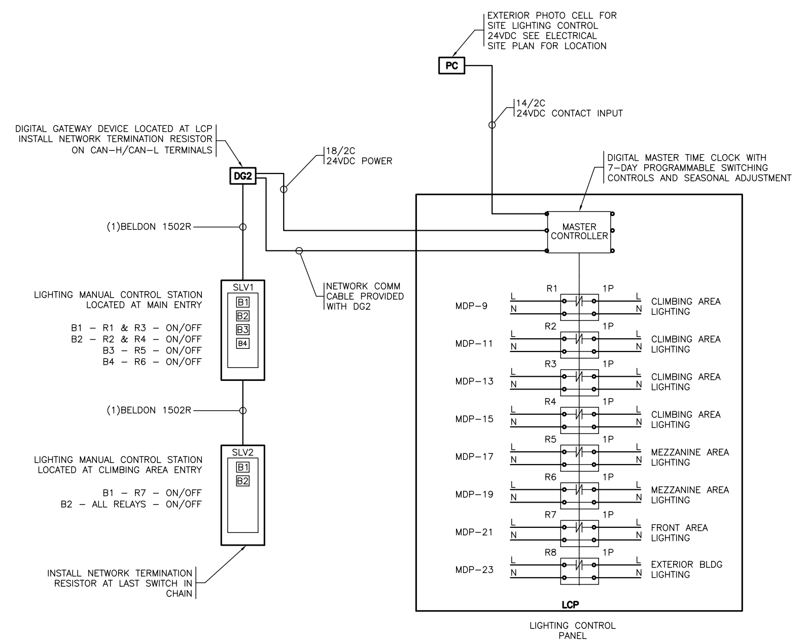
2 LIGHTING CONTROL DETAIL NOT TO SCALE
