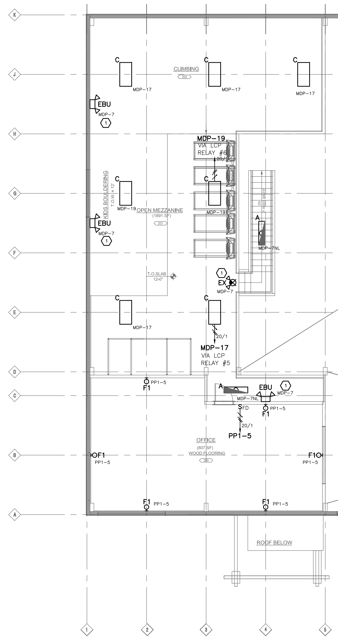
2 MEZZANINE PLAN 1/8"=1'-0"
