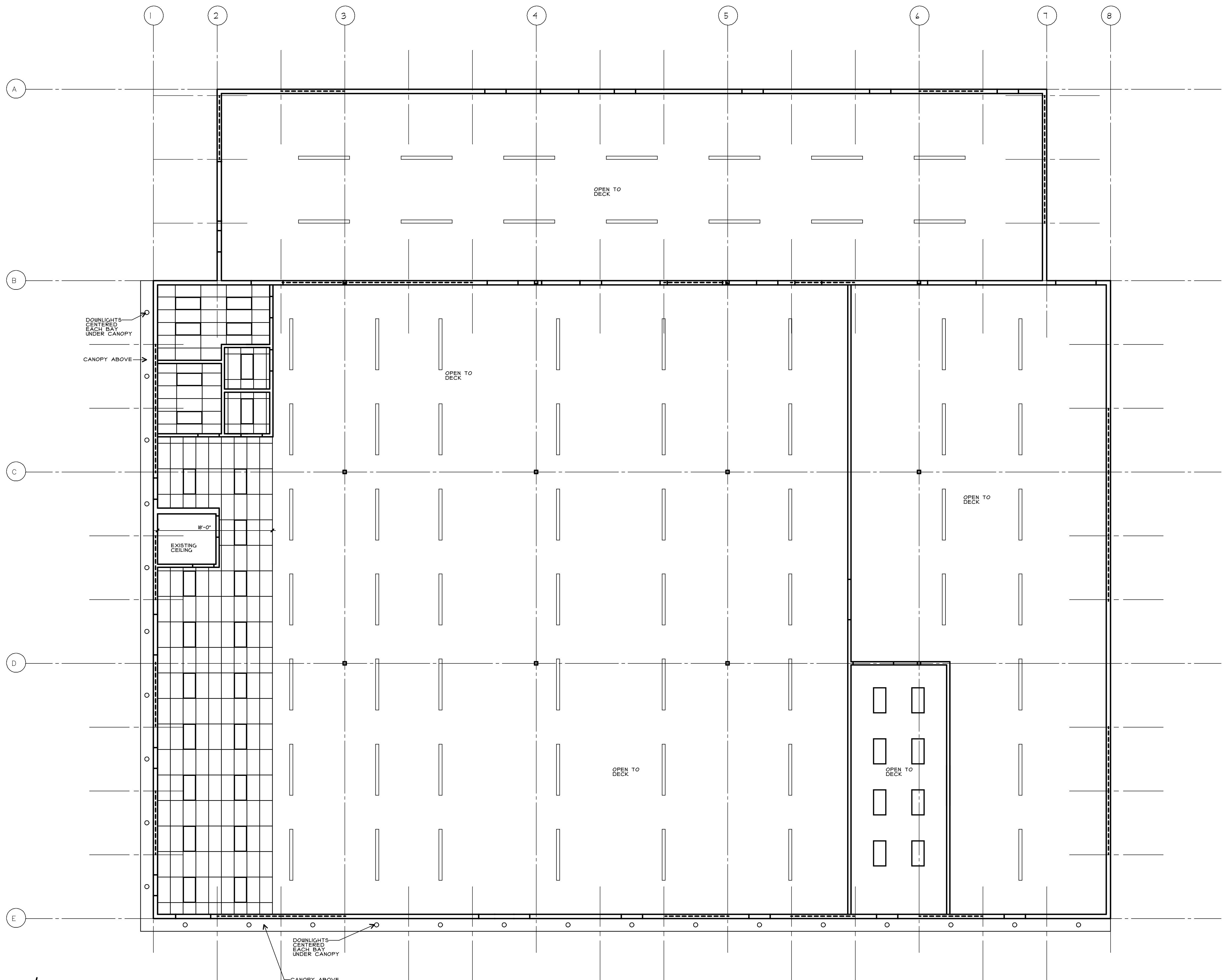
REFLECTED CEILING PLAN 1/8" = 1'-0"
