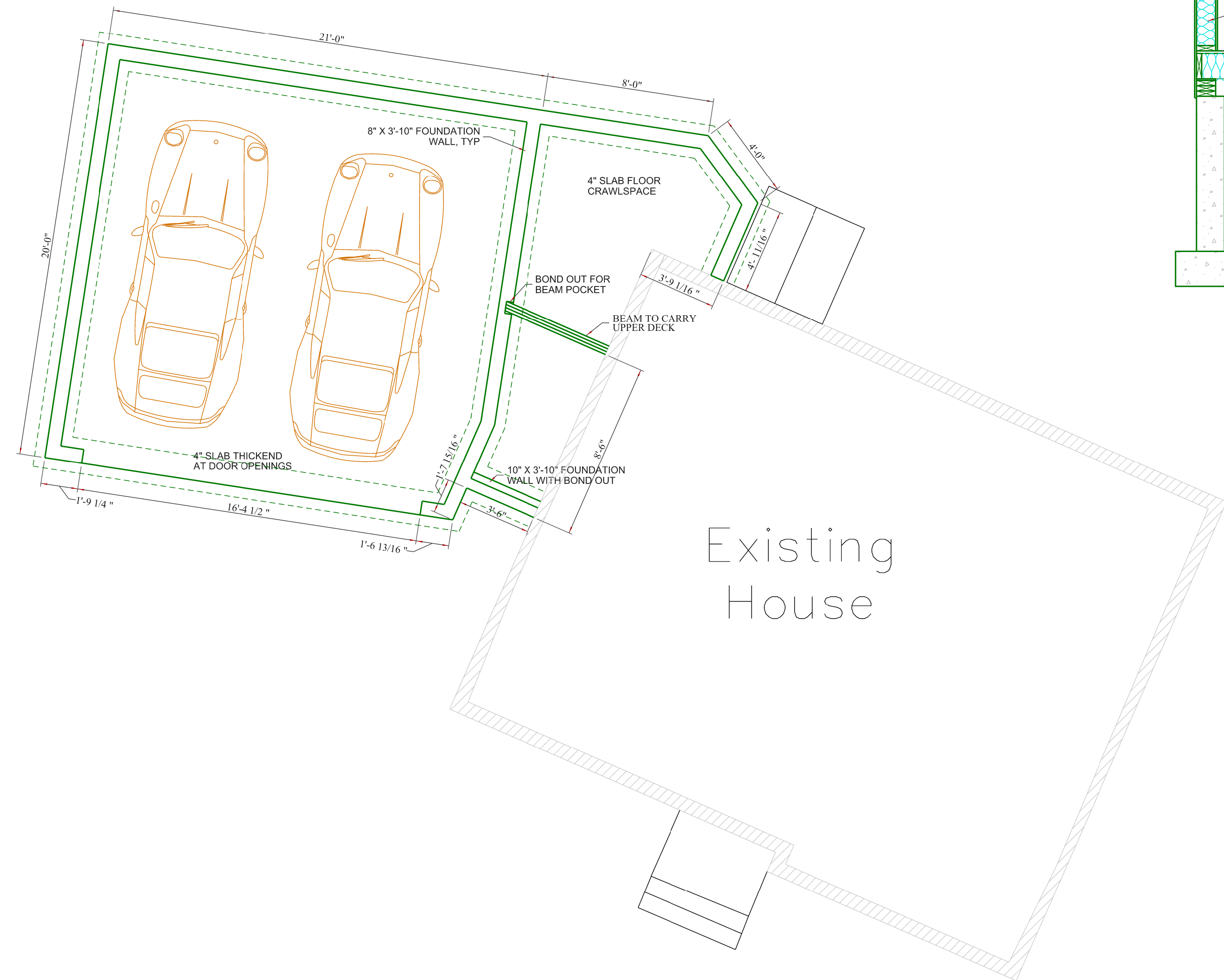
PROPOSED FOUNDATION PLAN SCALE 1/4"=1'-0"
