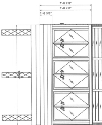
Front Elevation
