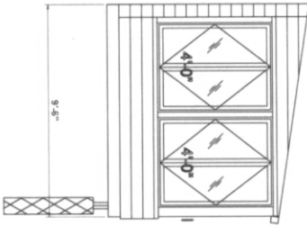
Left Elevation
