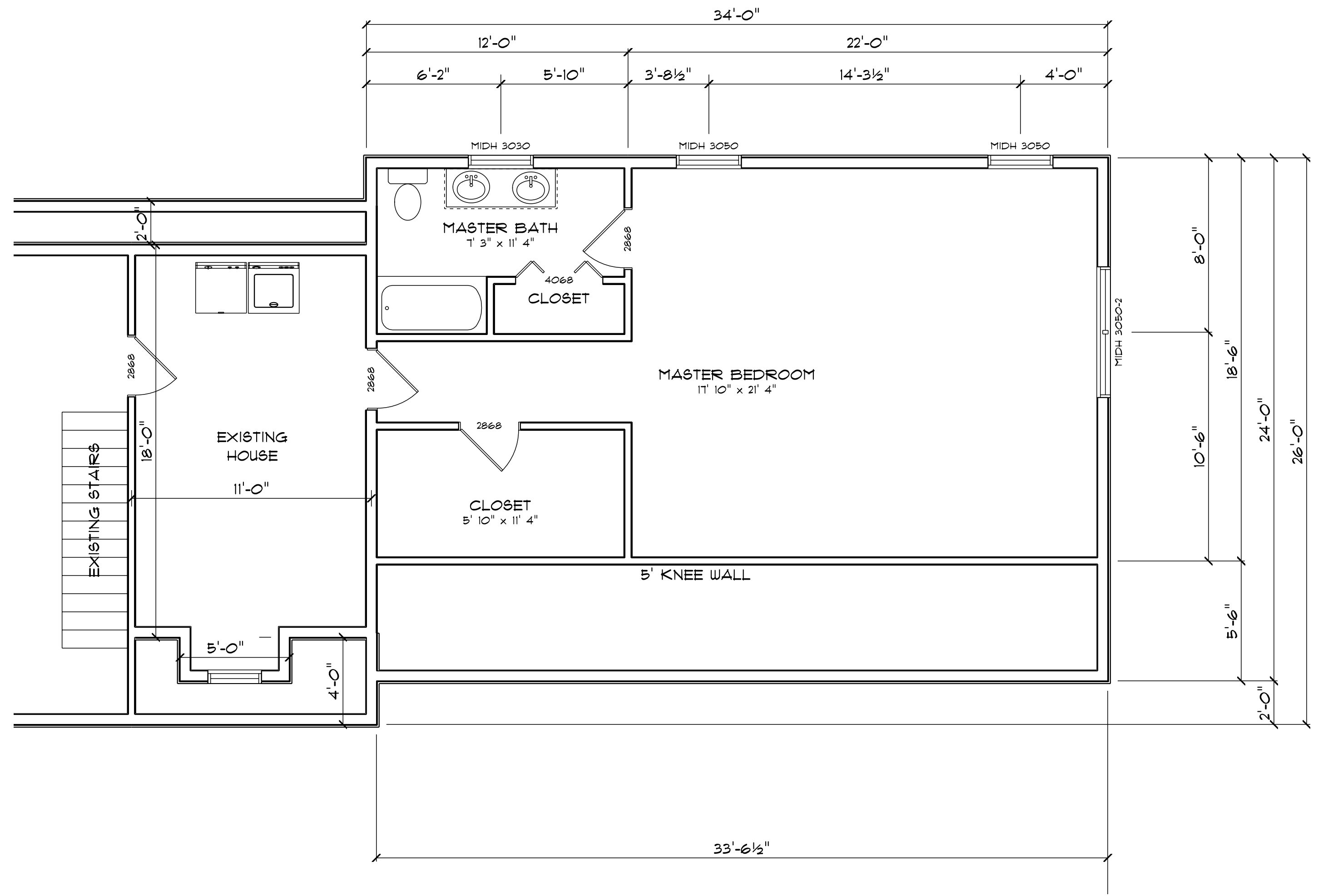
SECOND FLOOR SCALE: 1/4" = 1'-0"
