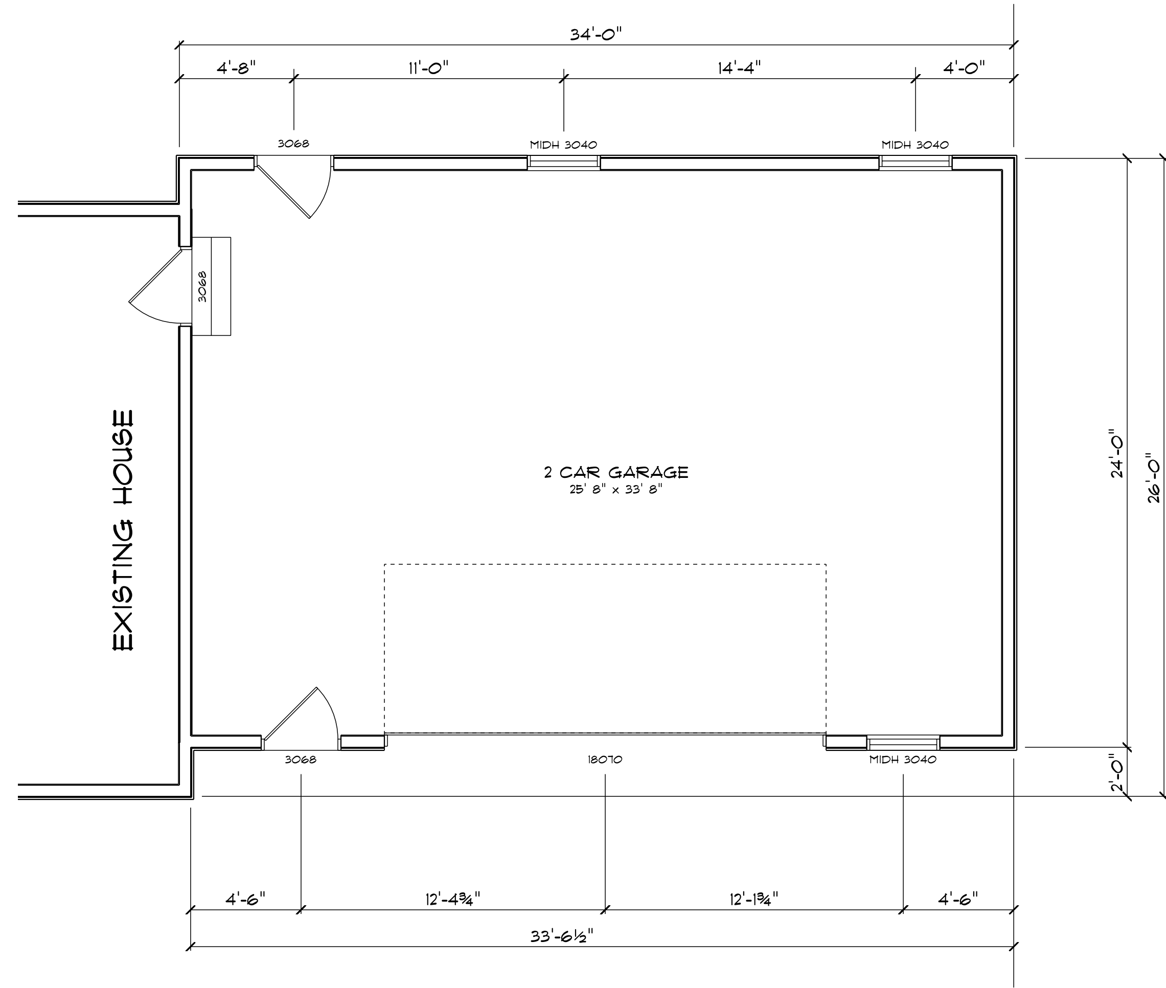
FIRST FLOOR SCALE: 1/4" = 1'-0"
