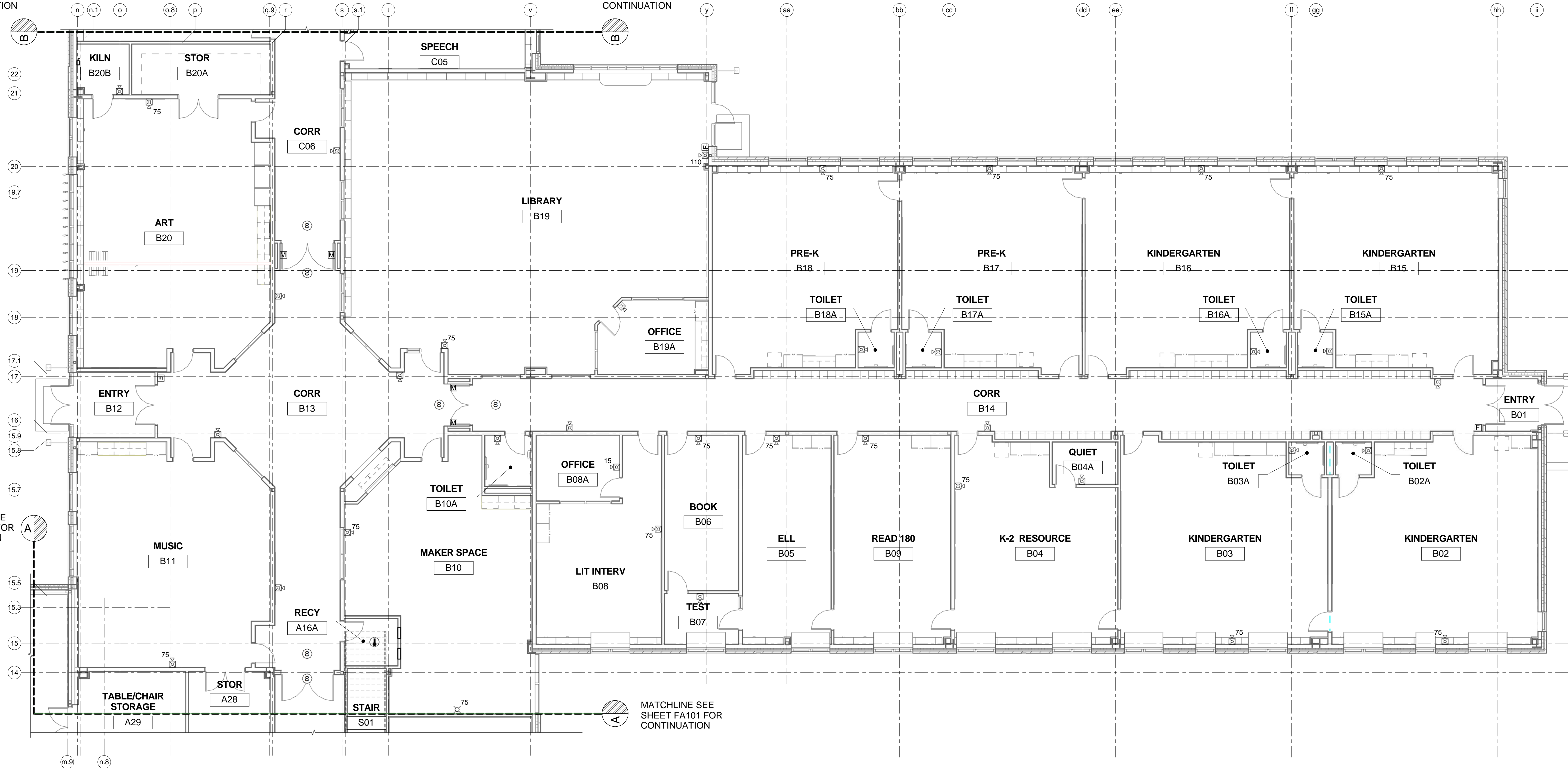
1 FIRST FLOOR FIRE ALARM PART PLAN B FA102 SCALE: 1/8" = 1'-0"
