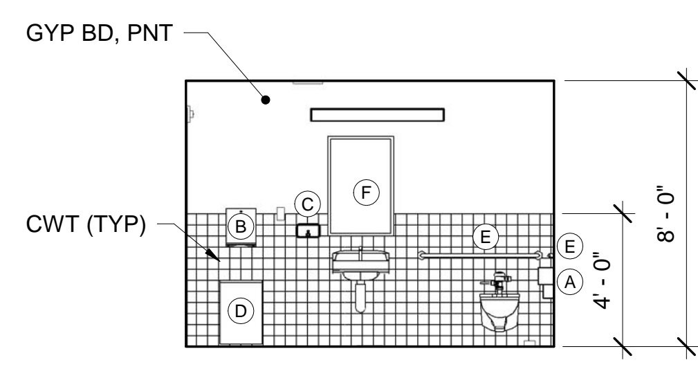
13 TOILET ROOM A39 - SOUTH ELEV AE422 AE422 SCALE: 1/4" = 1'-0"
