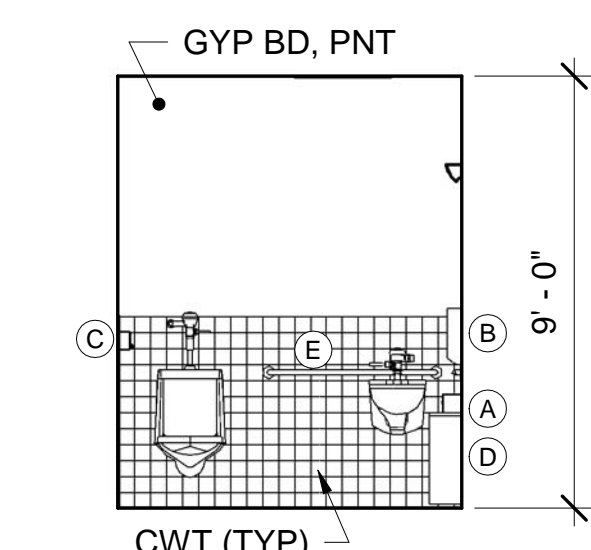
10 TOILET ROOM D09 - EAST ELEV AE422 AE422 SCALE: 1/4" = 1'-0"
