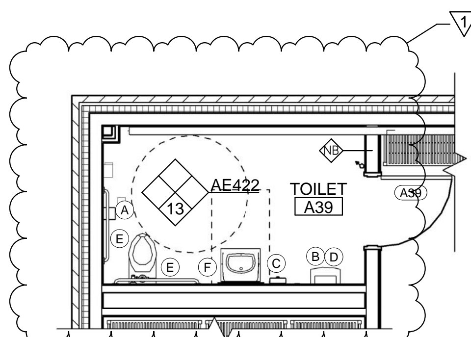
12 ENLARGED TOILET ROOM A39 PLAN AE101 AE422 SCALE: 1/4" = 1'-0"
