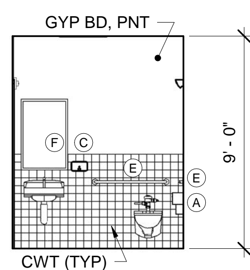
8 TOILET ROOM D36 - WEST ELEV AE422 AE422 SCALE: 1/4" = 1'-0"
