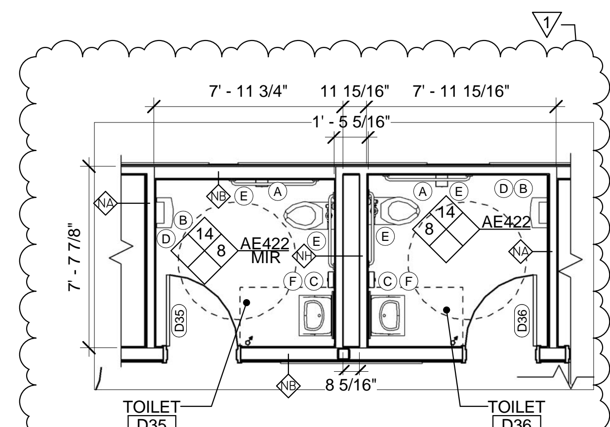
7 ENLARGED TOILET ROOM D35 AND D36 PLAN AE104 AE422 SCALE: 1/4" = 1'-0"
