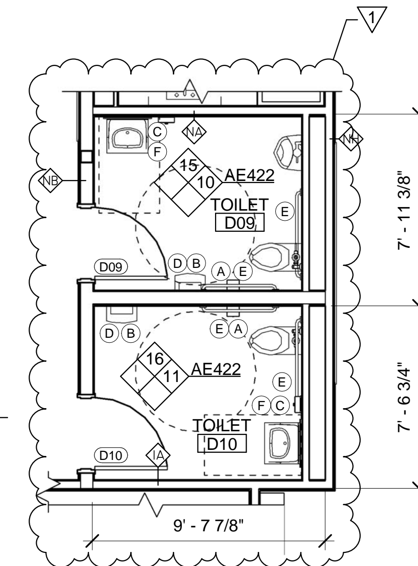
9 ENLARGED TOILET ROOM D09 AND D10 PLAN AE104 AE422 SCALE: 1/4" = 1'-0"
