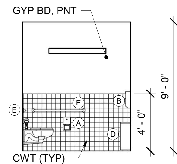
14 TOILET ROOM D36 - NORTH ELEV AE422 AE422 SCALE: 1/4" = 1'-0"
