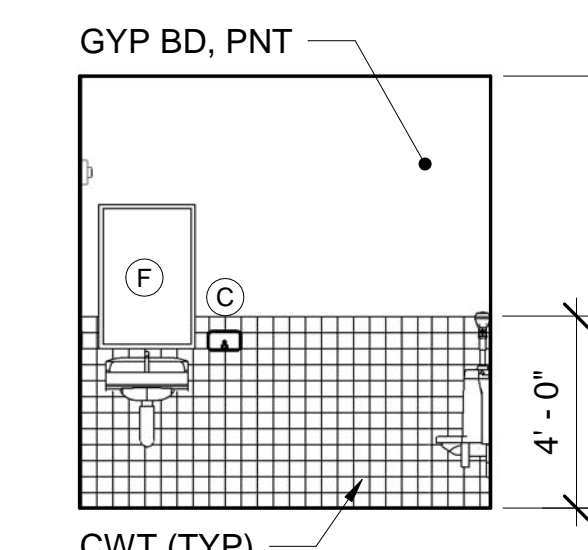
15 TOILET ROOM D09 - NORTH ELEV AE105 AE422 SCALE: 1/4" = 1'-0"
