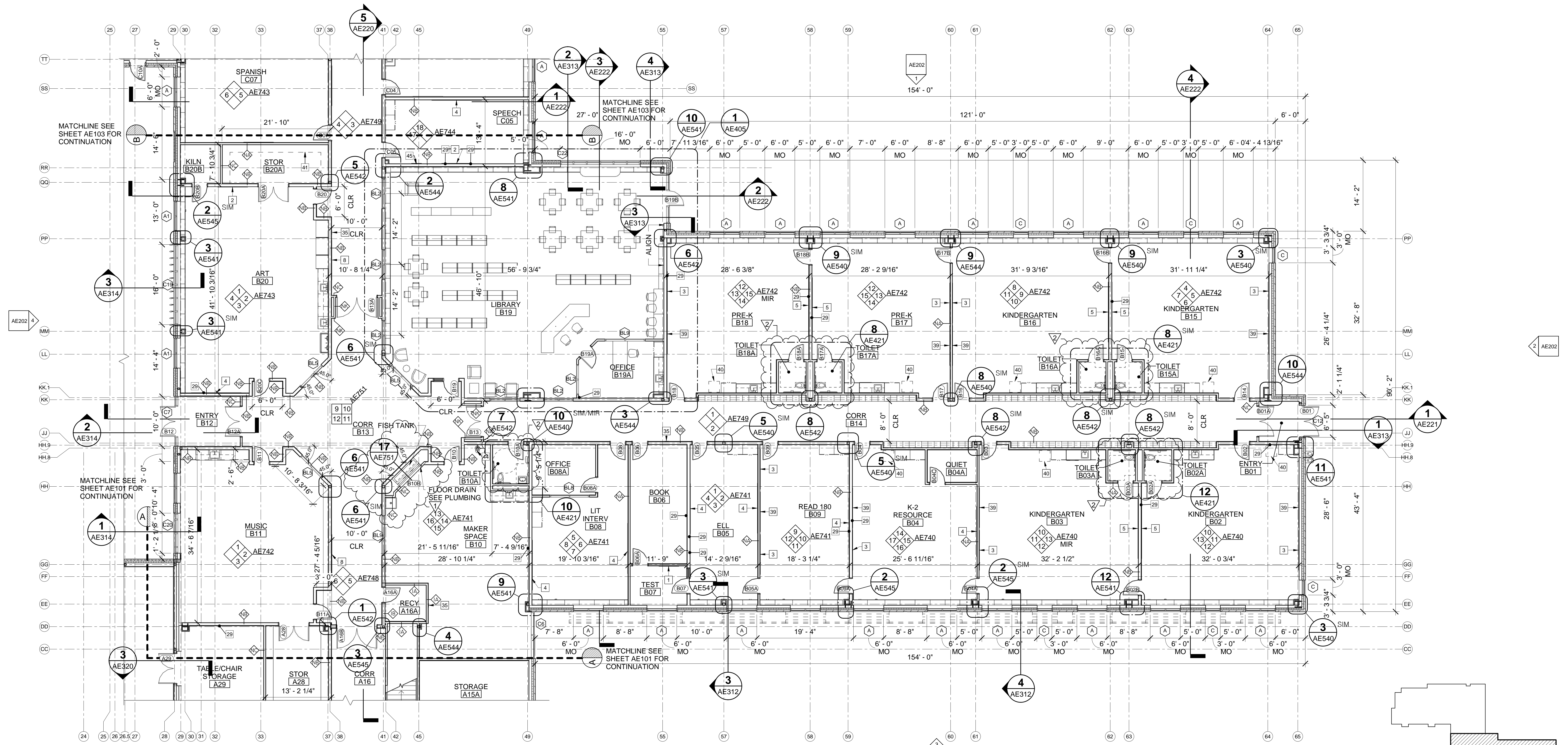
1 FIRST FLOOR PART PLAN WING B AE102 SCALE: 1/8" = 1'-0"
