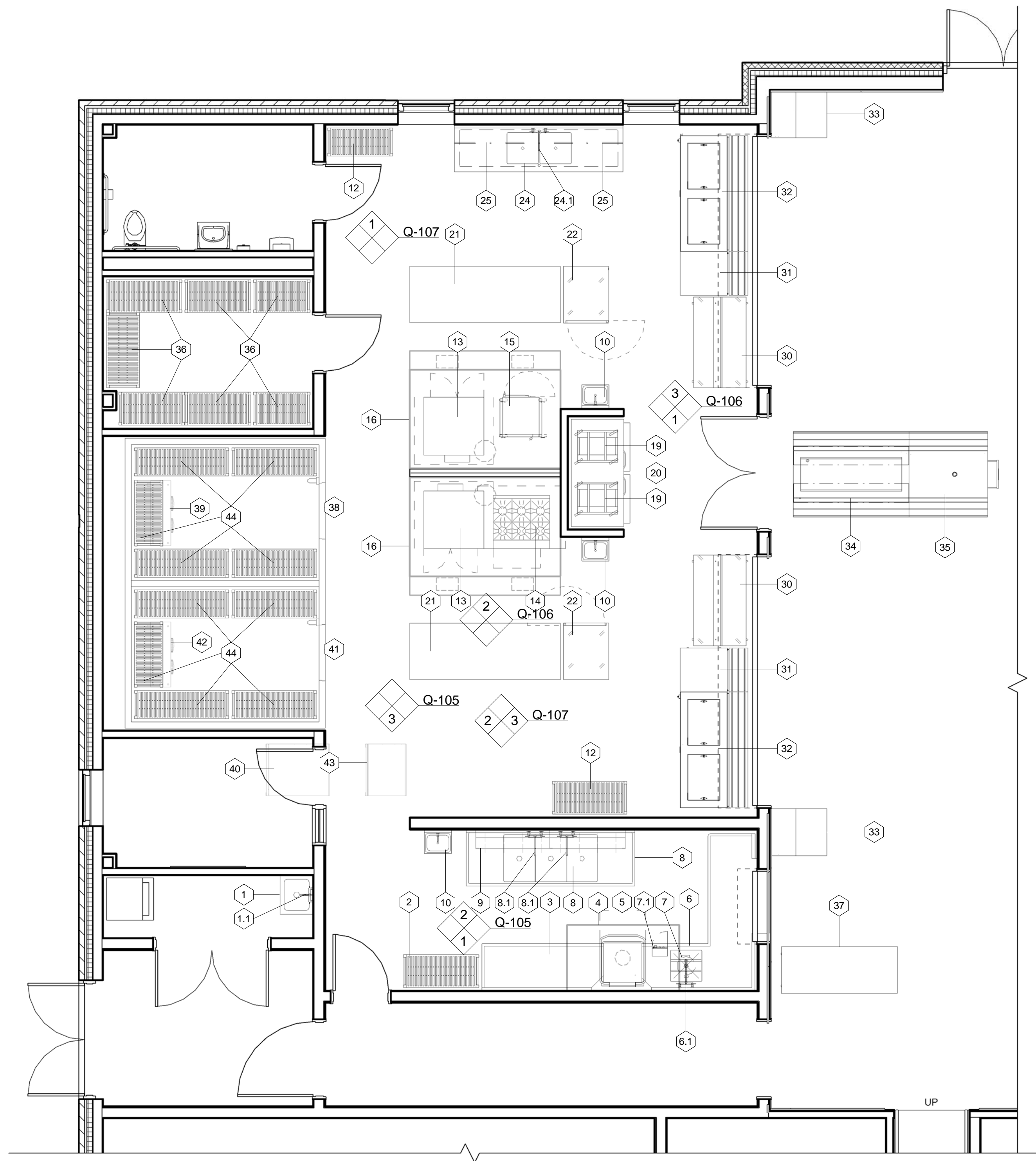
1 Foodservice Equipment Plan Q-101 SCALE: 1/4" = 1'-0"
