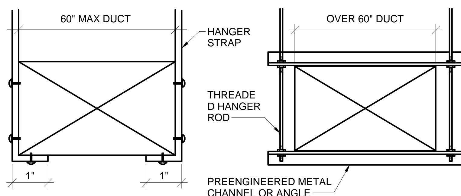
14 DUCT SUPPORT ATTACHMENTS DETAIL M-502/ SCALE: N.T.S.
