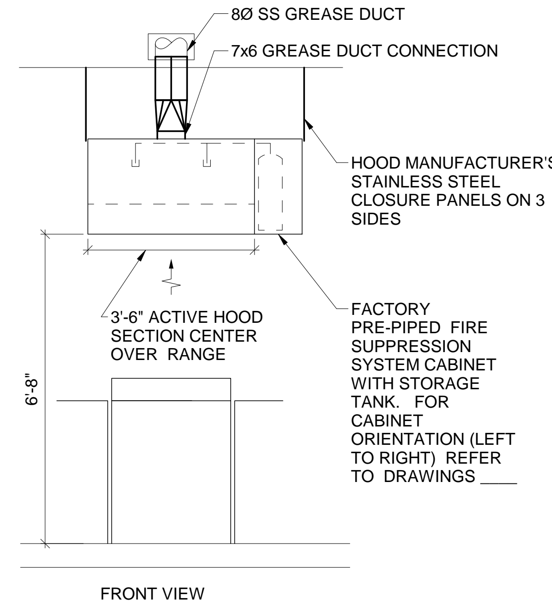
15 TYPICAL RANGE HOOD INSTALLATION DETAIL M-502/ SCALE: 1/8\"/>
