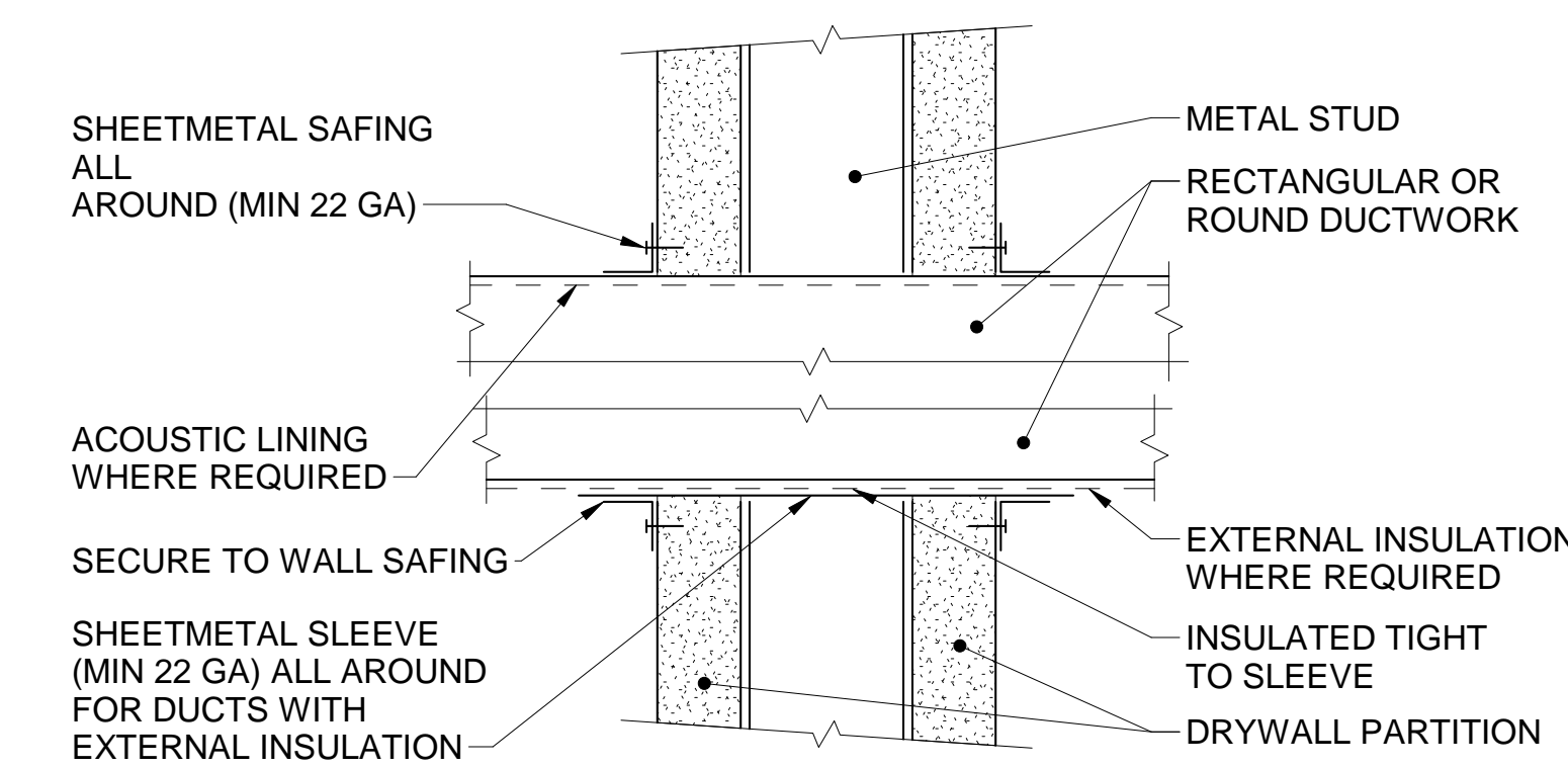
12 DUCT PENETRATION THRU NON-FIRE RATED WALL M-502/ SCALE: N.T.S.
