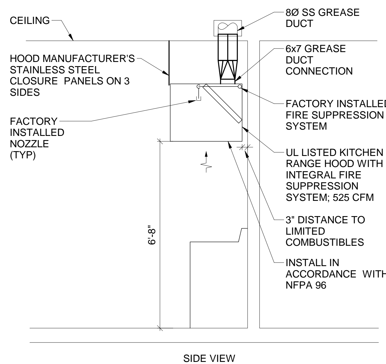
15 TYPICAL RANGE HOOD INSTALLATION DETAIL M-502/ SCALE: 1/8\"/>
