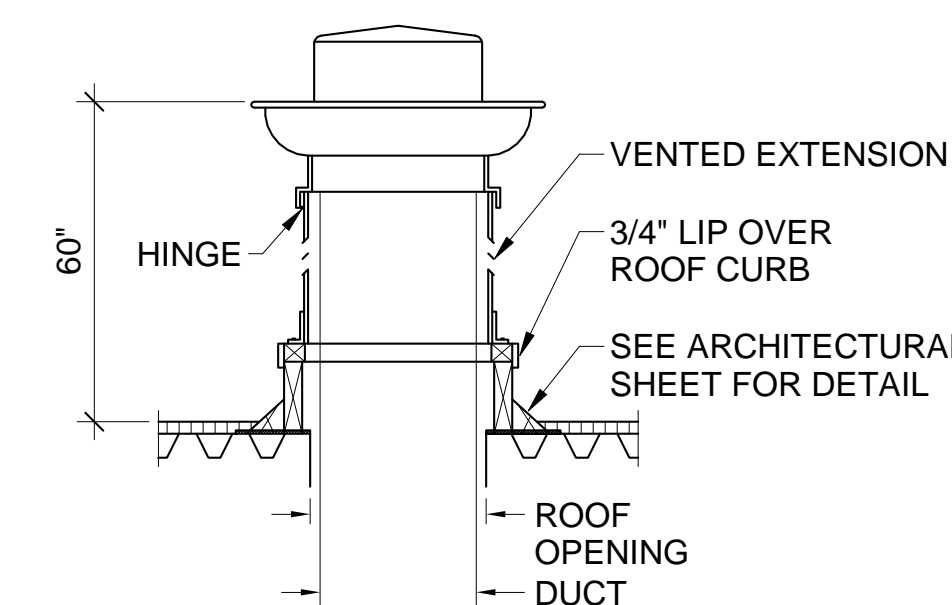
8 KITCHEN EXHAUST HOOD FAN ROOF CURB M-502/ SCALE: N.T.S.
