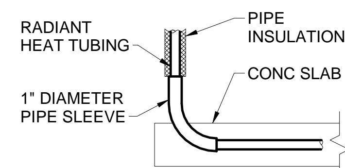
11 TYPICAL RADIANT HEAT TUBING ENTERING OR EXITING CONCRETE SLAB DETAIL M-502/ SCALE: N.T.S.
