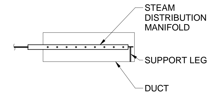
9 DUCT MOUNTED HUMIDIFIER MANIFOLD PIPING SCHEMATIC M-502/ SCALE: N.T.S.
