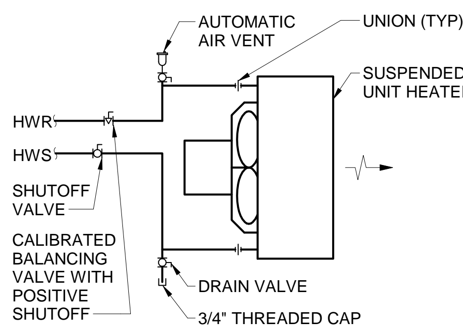
7 UNIT HEATER WATER COIL PIPING SCHEMATIC M-502/ SCALE: N.T.S.
