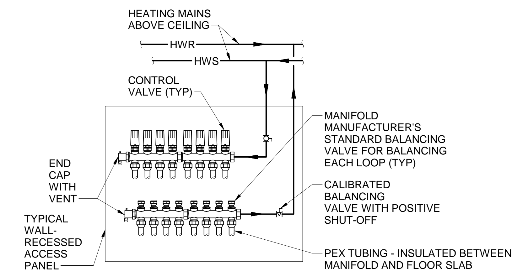
10 TYPICAL RADIANT HEAT MANIFOLD DIAGRAM M-502/ SCALE: N.T.S.
