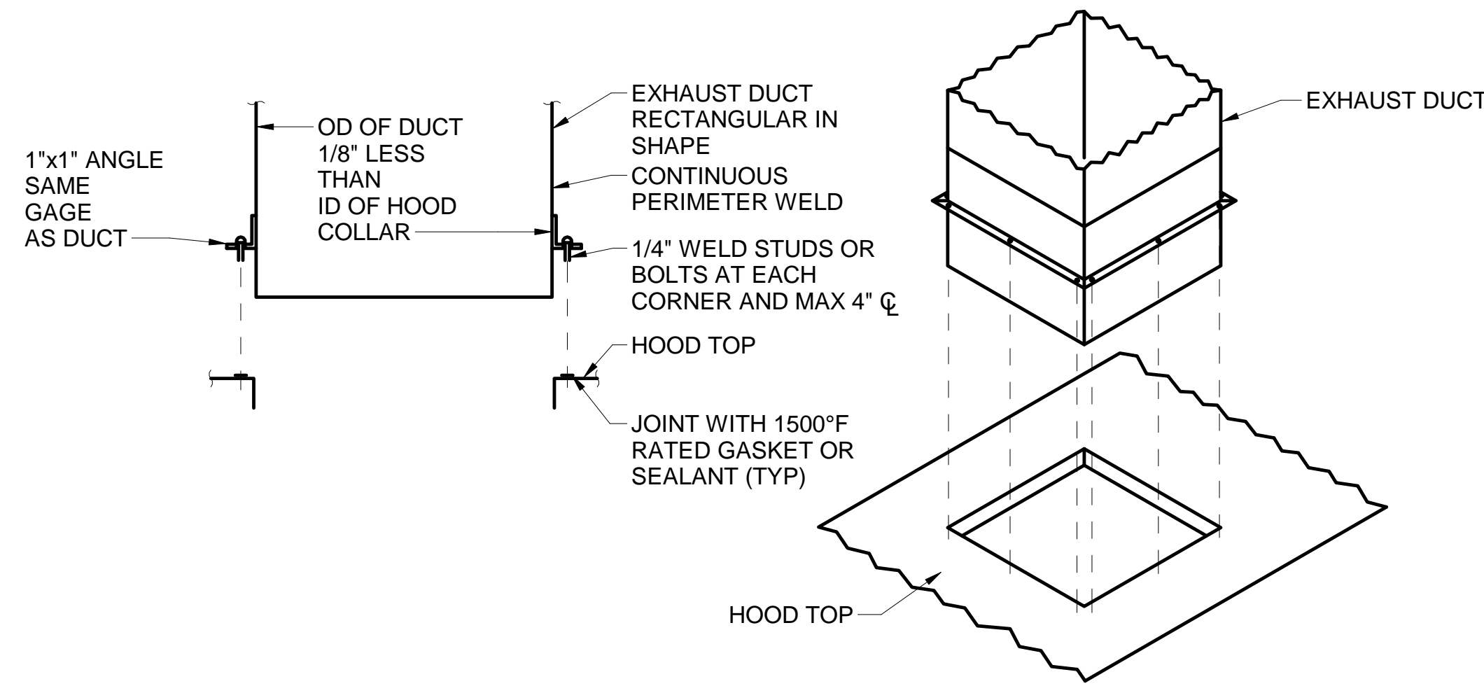
2 KITCHEN HOOD DUCT CONNECTION M-502/ SCALE: N.T.S.
