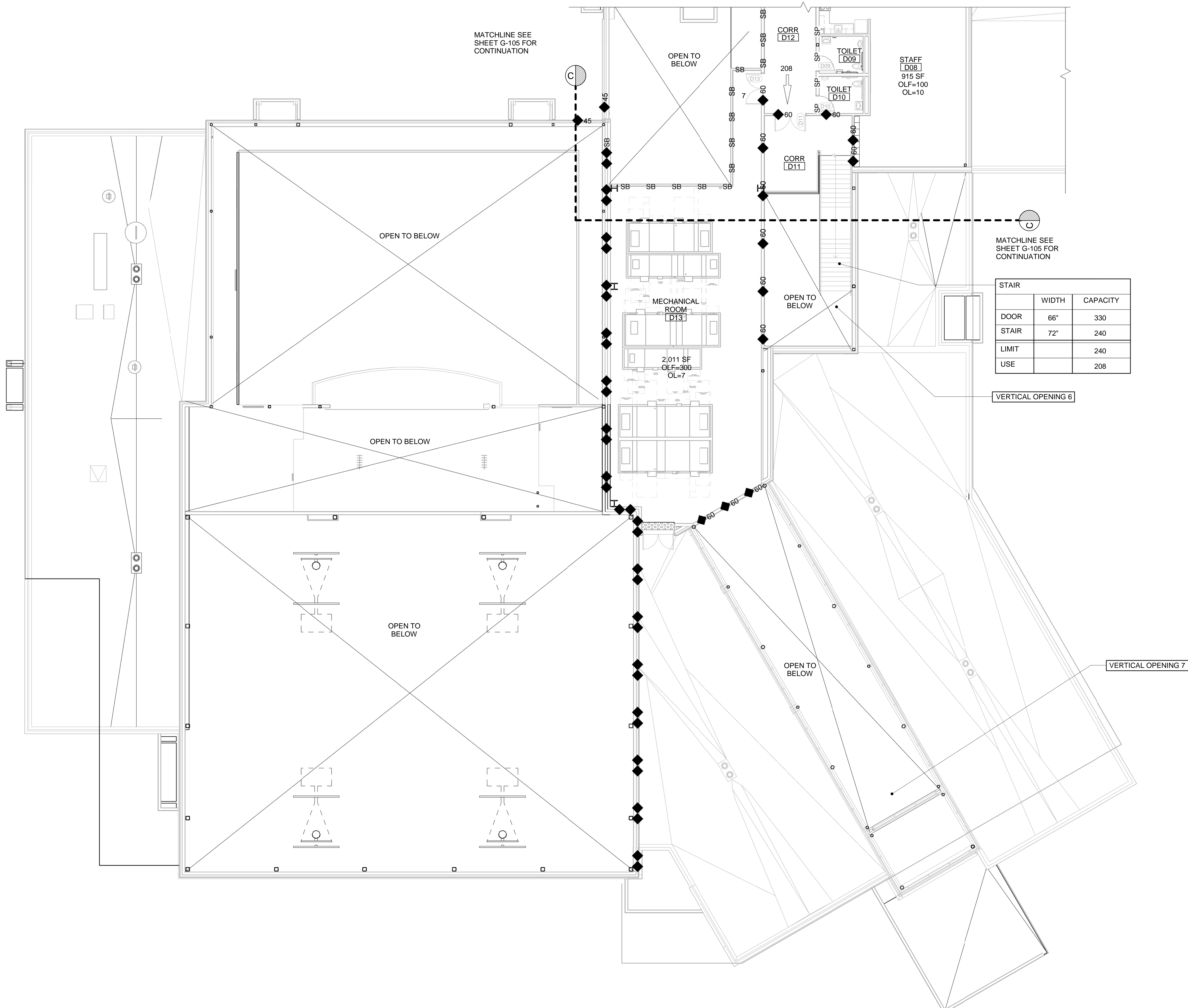
1 EGRESS AND FIRE RATING SECOND FLOOR PART PLAN WING D - SOUTH END G-106 SCALE: 1/8" = 1'-0"
