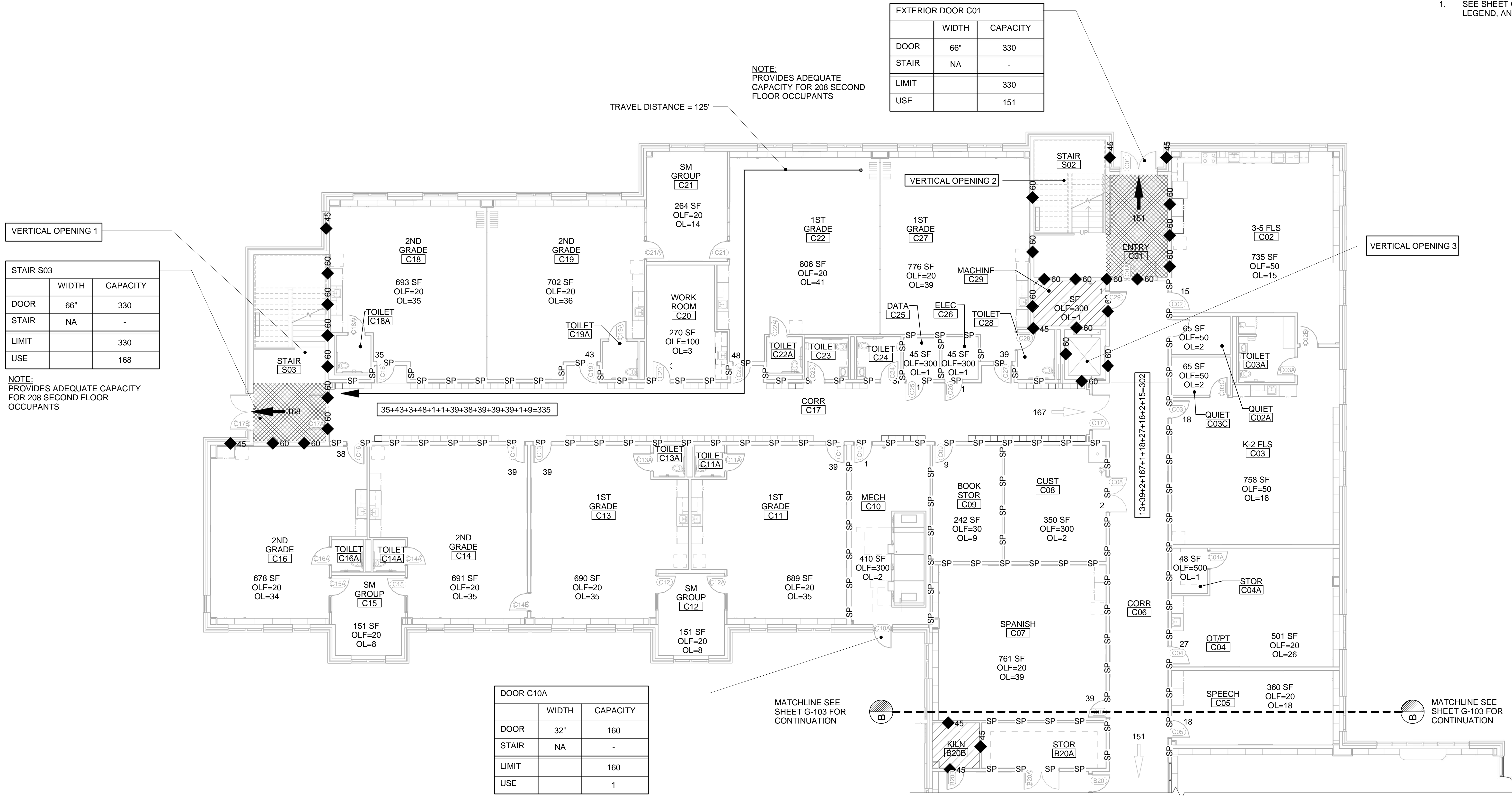
1 EGRESS AND FIRE RATING FIRST FLOOR PART PLAN WING C G-104 / SCALE: 1/8" = 1'-0"
