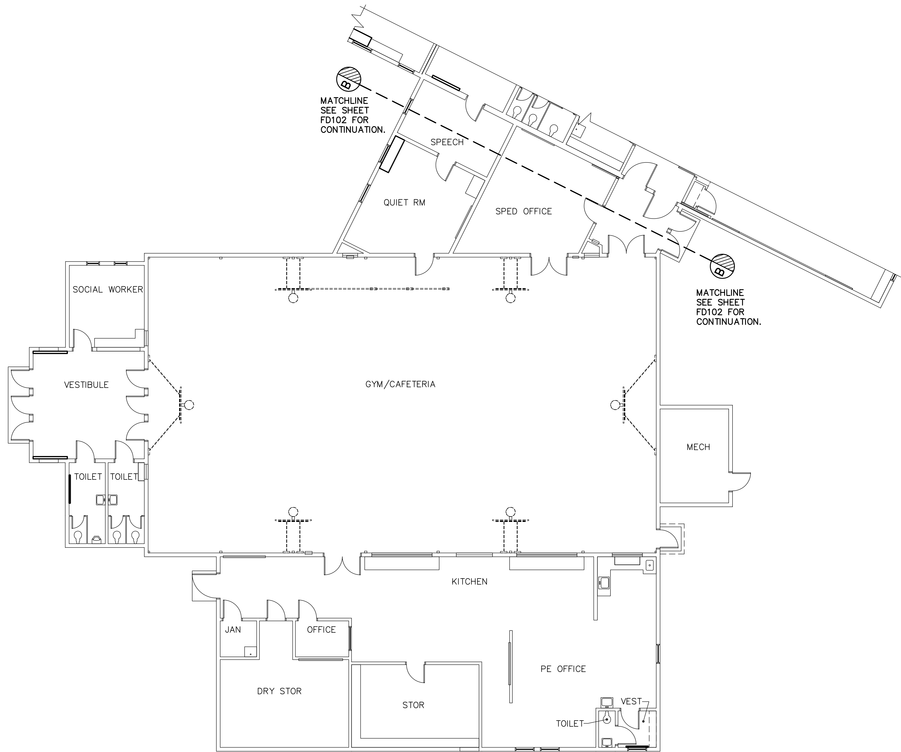
1 FIRE SUPPRESSION REMOVALS PART PLAN FD103 SCALE: 1/8"=1'-0" PLAN NORTH
