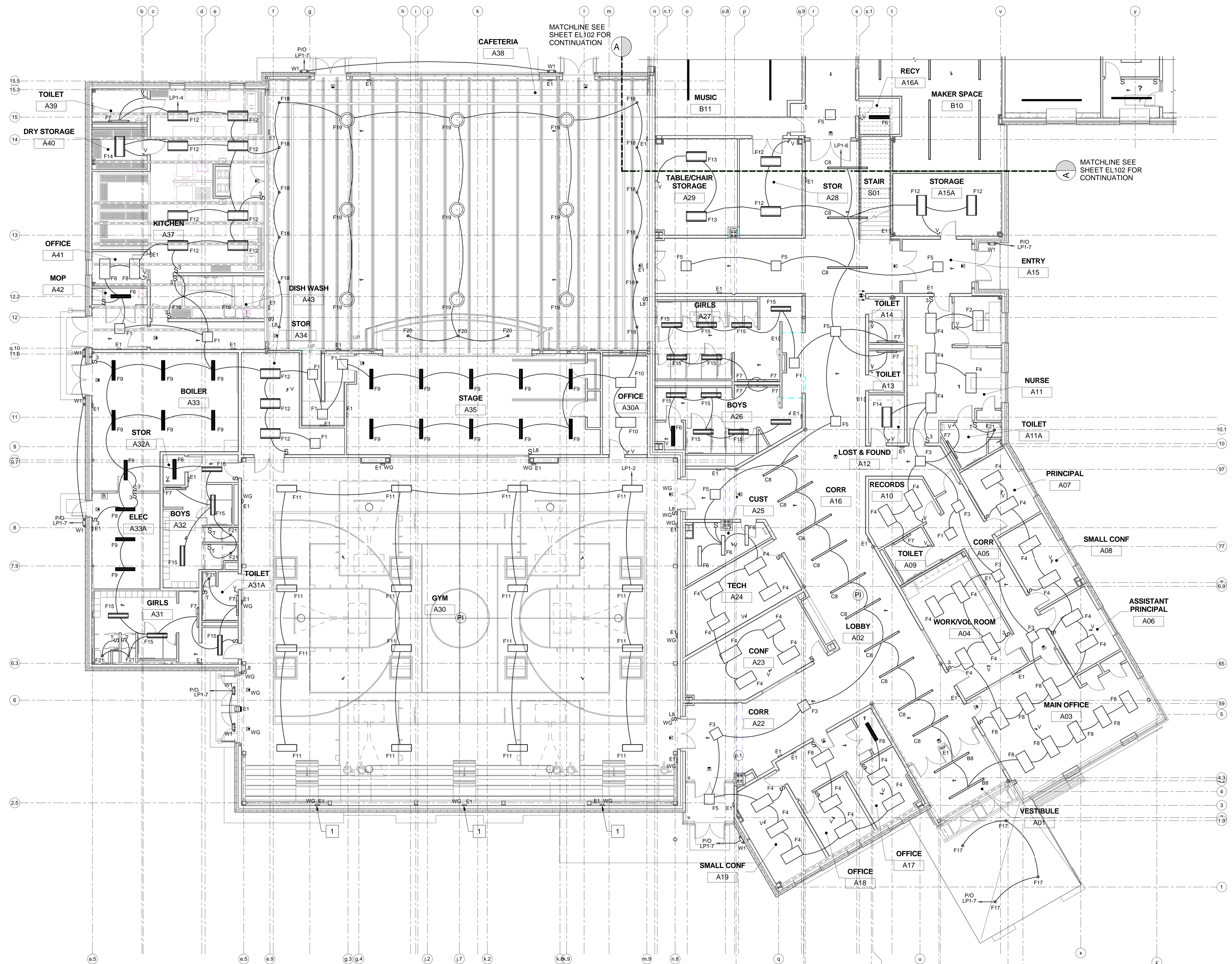
1 FIRST FLOOR LIGHTING PART PLAN A EL101 SCALE: 1/8" = 1'-0"
